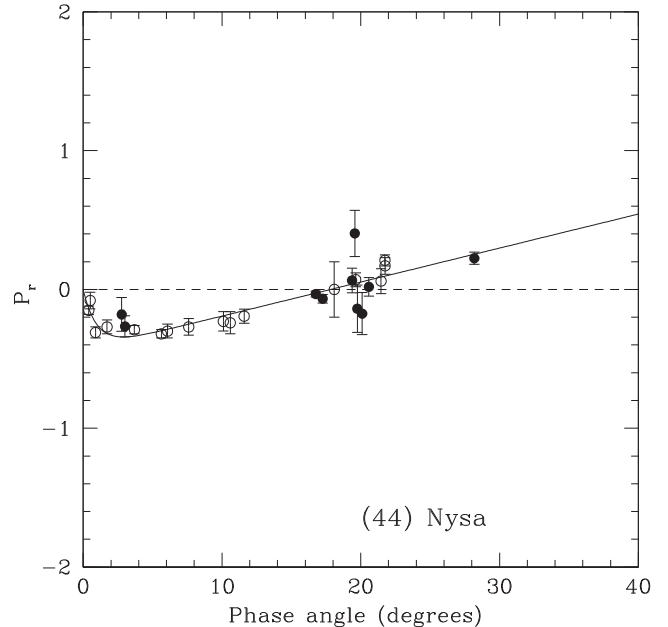
Figure 1. The phase–polarization curve of the high-albedo asteroid (44) Nysa. In this and other figures, full symbols indicate measurements taken at the Complejo Astronómico El Leoncito (CASLEO, Argentina) observatory and recently published by Gil-Hutton et al. (2014). Open symbols are other measurements taken from the literature. The solid curve is the best-fitting curve using the exponential–linear representation (Equation 2).
