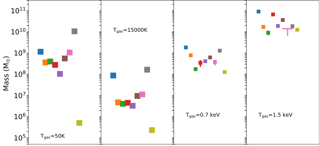
Figure 1. Visualisation of mass-temperature profile presented in Table 1, with the coolest molecular gas from the left and the hot ambient ICM at 1.5 keV from the right. Within each panel, we shift the data points horizontally for clarity and the clusters are presented in the same order as the first column in Table 1, i.e. 2A0335+096 is on the left and Virgo is on the right.
