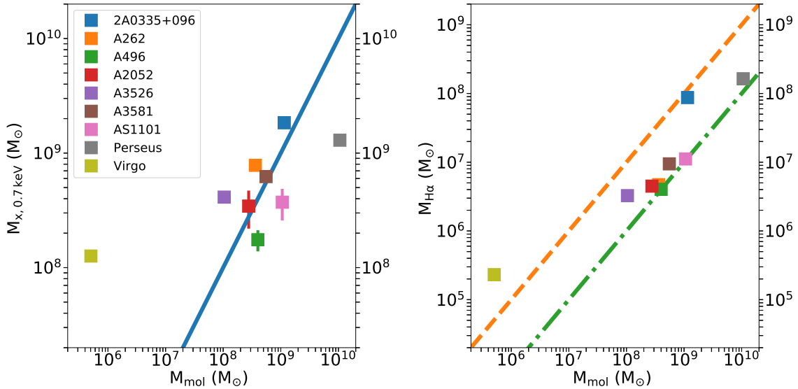
Figure 2. Left: The X-ray emitting gas against molecular mass. The blue line indicates where the molecular mass would match the soft X-ray mass. Right: The mass of \text{H}\alpha component against molecular mass. The orange dash line has a constant M_{\text{H}\alpha}/M_{\text{mol}} ratio of 0.1 and the green dash-dot line has a ratio of 0.01. The uncertainties in the mass of molecular and \text{H}\alpha emitting gas is smaller than the marker size.
