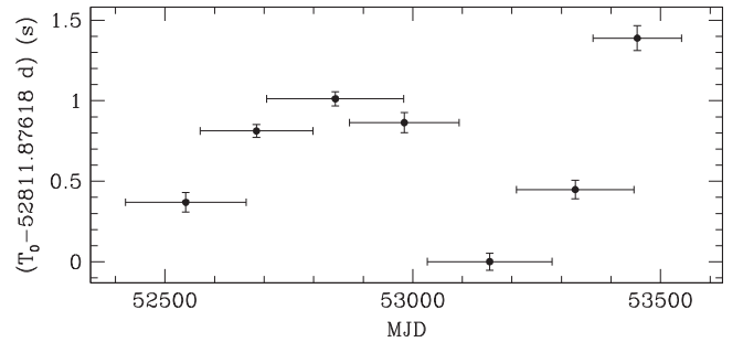
Figure 2. Variation of the time of passage through ascending node (orbital phase 0), computed for overlapping segments of data and holding all other timing parameters fixed at their nominal values.
