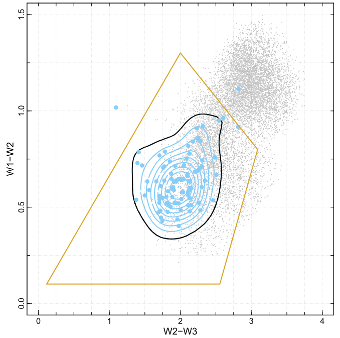
Figure 3. WISE W2-W3 vs. W1-W2 color-color diagram. The 93 sources in the training set are shown by light blue circles, and the black line is the contour containing 90% of the sources in the training set and used to select the candidate KDE BL Lacs. Sources in the WIRaLS catalog are displayed in the background for comparison (small gray circles). The yellow polygon shows the region in the WISE color plane where sources from the 2WHSP catalog are located (Chang et al. 2017; see Section 5.1).
