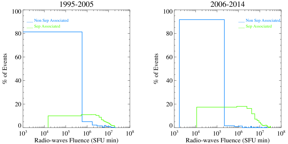
Fig. 4.— Radio fluence probability density functions: 1995-2005 database (left panel) and 2006-2014 database (right panel)
