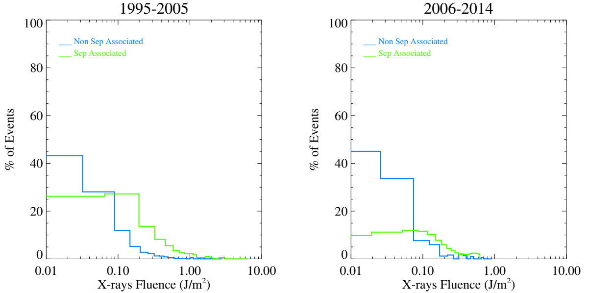
Fig. 3.— SXR fluence probability density functions: 1995-2005 database (left panel) and 2006-2014 database (right panel)
