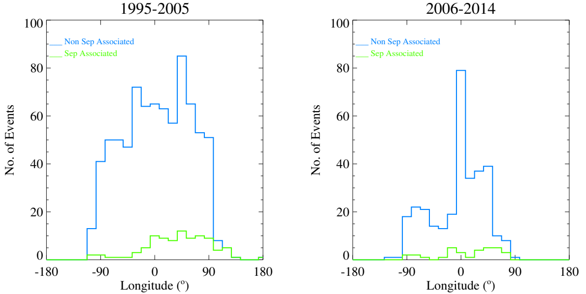
Fig. 5.— Longitudinal distributions of flare locations: 1995-2005 database (left panel) and 2006-2014 database (right panel)
