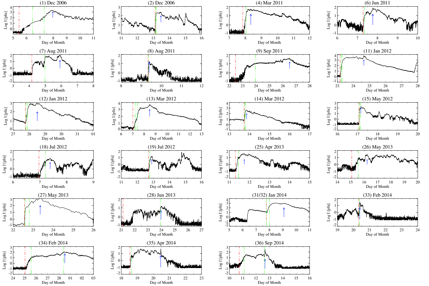
Fig. 1.— Proton flux as measured by GOES spacecraft for the \geq M2 flare events in Table 1. The red line evidences the time when the forecast is made, while the next two green lines refer to 10 pfu and 100 pfu threshold crossings. Finally, a blue arrow is used to show the maximum of each event.
