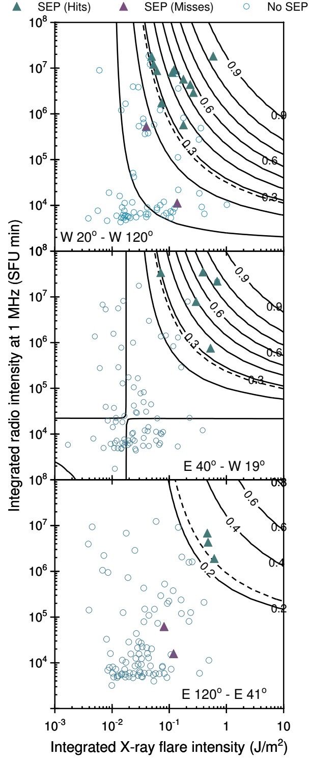
Fig. 6.— Probability contours for SEP forecasting for three different longitudinal bands: SEPs hit (green triangles), SEPs miss (violet triangles) and No SEPs associated (circles).
