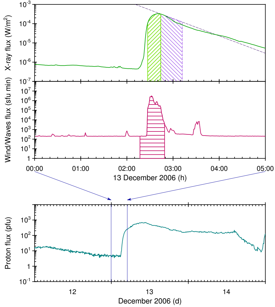
Fig. 2.— Key parameters for the 2006 December 13 SEP event. From top to bottom: X-ray flux, Radio Waves flux and Proton flux.
