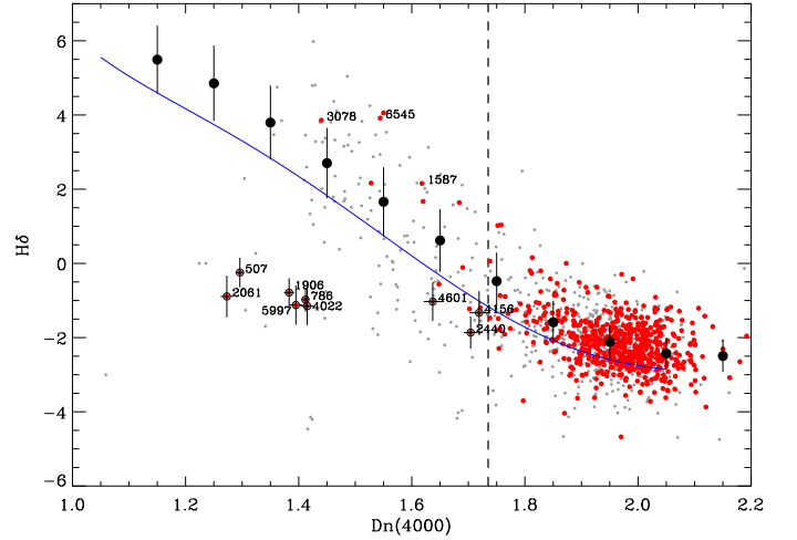
Fig. 4. H\delta index versus D_n(4000) diagram. Black filled circles represent the relationship derived for the MPA-JHU sample that is shown in Fig. 2. The blue line is a polynomial fit to the 1-\sigma limit of this relationship. All objects above this line are considered E+A contaminants. Gray dots refer to the sources in the BH12-A sample with z \leq 0.1 and S/N > 2 in the W2 and W3 bands. Red dots highlight the objects with the emission line EW < 5 \text{ \AA} and a FIRST central counterpart. Red dots circled in black are the nine BL Lacs candidates. The vertical dashed line indicates the limit D_{n_{\max}} = 1.735 .
