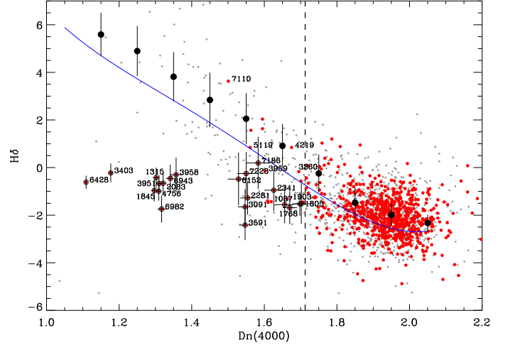
Fig. 8. Same as Fig. 4, but for 0.1 < z \leq 0.15 .
