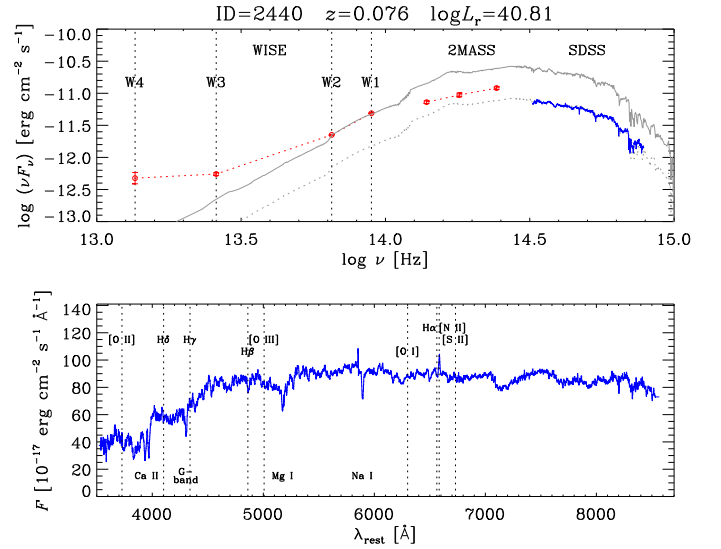
Fig. 5. Top: SED of a new BL Lac candidate, ID=2440. Red circles display WISE and dereddened 2MASS flux densities. The SDSS dereddened spectrum is shown in blue. Gray lines represent two SWIRE templates of a 13 Gyr old elliptical galaxy normalized to the W2 band (solid) or to the SDSS spectrum (dotted). The departure of the SDSS spectrum from the latter template highlights the reduced Dn(4000) value of the source, while the W3 (and W4) excess appears from the comparison of the WISE data with the first template. Bottom: rest-frame SDSS spectrum with indication of the main AGN emission lines (upper labels) and galactic absorption lines (lower labels).
