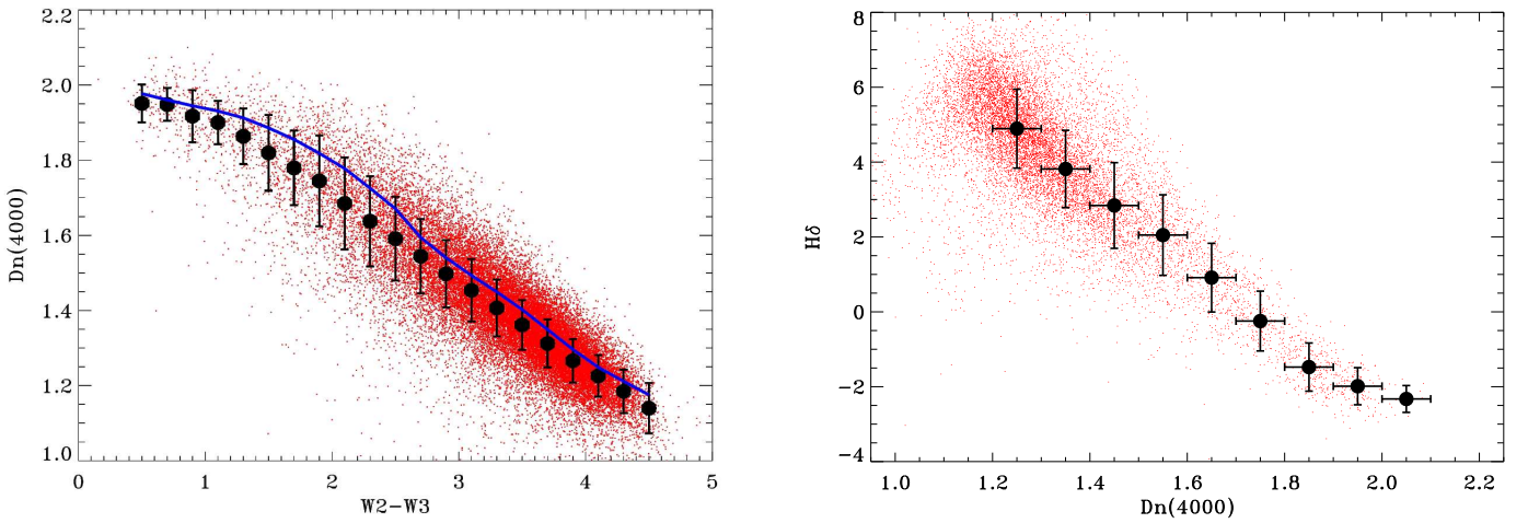
Fig. 6. Same as Fig. 1 (left panel) and Fig. 2 (left panel), but for 0.1 < z \leq 0.15 .
