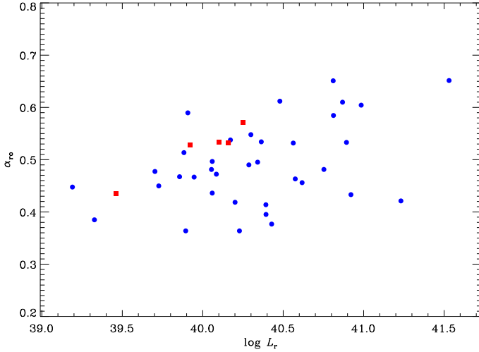
Fig. 10. Radio-optical spectral index \alpha_{10} versus the logarithm of the radio luminosity L_r for the 36 BL Lac candidates in the “forbidden” zone of the Dn(4000) versus W2-W3 diagram (blue dots). The red squares correspond to the five objects located in the “wedge” region of the same diagram.
