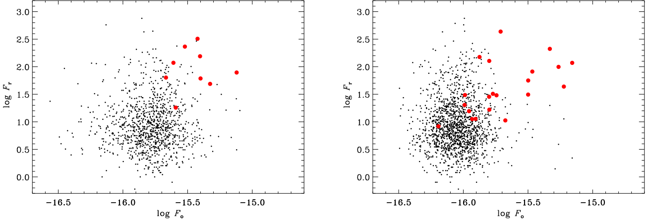
Fig. 14. Left panel: the flux density of the FIRST central component, F_r , versus dereddened flux density within the SDSS fiber at 3900 Å, F_o , for the sources with 0.05 < z \leq 0.1 . The candidate BL Lacs are plotted with red circles. Right panel: same as in the left panel, but for 0.1 < z \leq 0.15 .
