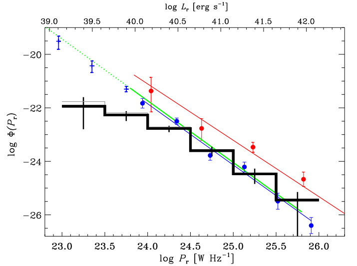
Fig. 16. RLF at 5 GHz of the selected BL Lac candidates (black histogram). The gray histogram shows the effects of including the five objects located in the “wedge”. The results from Padovani et al. (2007) are in red, while blue dots refer to the work by Marchã & Caccianiga (2013) for “classical BL Lacs”. We also report (as plus signs) three points at low luminosity of the Marchã & Caccianiga RLF for “Type 0” AGNs. The green line is the RLF normalized to match the number of objects of our sample with \log P_r > 23.8 [\text{W Hz}^{-1}] , after having adopted the same slope of Marchã & Caccianiga (2013).
