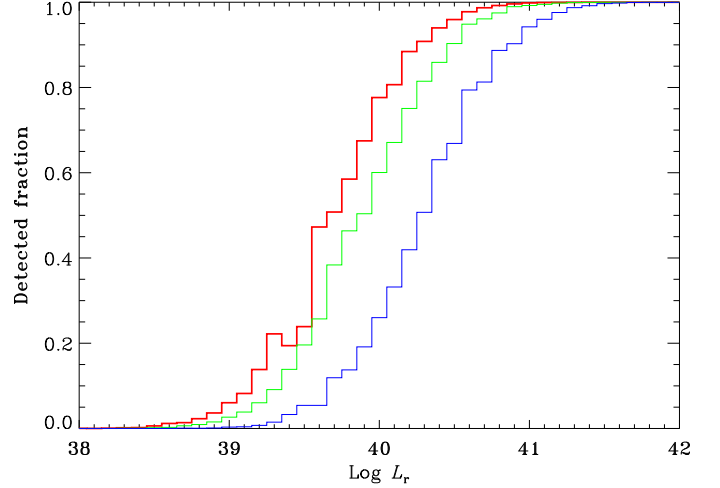
Fig. 15. Expected fraction of BL Lac candidates recovered with our selection method at various levels of radio luminosity obtained with Monte Carlo simulations. The various lines refer to different assumptions on the radio–optical spectral index. Red: \alpha_{r0} = 0.49 , the mean obtained from the 35 BL Lac candidates with 0.05 < z \leq 0.15 ; green: \alpha_{r0} = 0.53 , the mean of the candidates with \log L_r > 40.5 \text{ erg s}^{-1} ; blue: \alpha_{r0} = 0.59 , the mean of the 1Jy BL Lacs.
