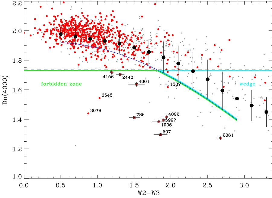
Fig. 3. D_n(4000) versus W2-W3 diagram. Black filled circles represent the relationship derived for the MPA-JHU sample that is shown in Fig. 1. The blue line is a polynomial fit to the 1-\sigma limit of this relationship. Gray dots represent the sources in the BH12-A sample with z \leq 0.1 and S/N > 2 in the W2 and W3 bands. Red dots highlight the objects with rest-frame emission line EW < 5 \text{ \AA} and a FIRST central counterpart. Red dots circled in black are the nine BL Lacs candidates, i.e. those sources with D_n(4000) < 1.735 (shown by the horizontal dashed line) that meet the additional constraint on the H\delta index (see Fig. 4). The boundaries of the “forbidden” zone and “wedge” region are highlighted with a green and a cyan line, respectively.
