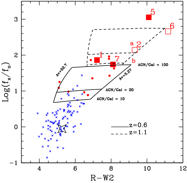
Figure 7. The f_x/f_o ratio as a function of the optical-IR colour for our EXO50 type 2 QSO objects and for the comparison sample. We also report the expectations from the toy model at z = 0.6 and 1.1 for two values of optical obscuration ( A_V = 5.27 and 52.7 corresponding to N_H \simeq 10^{22} and 10^{23} \text{ cm}^{-2} , respectively) and three values (10, 20, 100) of AGN/host ratio at \sim 4.6 \mu\text{m} ; the big star marks the position where the toy model converges for all the AGN/host ratio used here when N_H < \text{few times } 10^{20} \text{ cm}^{-2} (i.e. at the unabsorbed type 1 view). Symbols and colours are as in Fig. 4. The numbers mark our EXO50 objects as reported in Tables 1 and 3. The labels (a) and (b) mark the position of the objects XBSJ021642.3–043553 ( z \sim 2 , source a) and XID2028 ( z \sim 1.6 , source b) discussed in Section 5.2. See Section 5.6 for details on the modelling.
