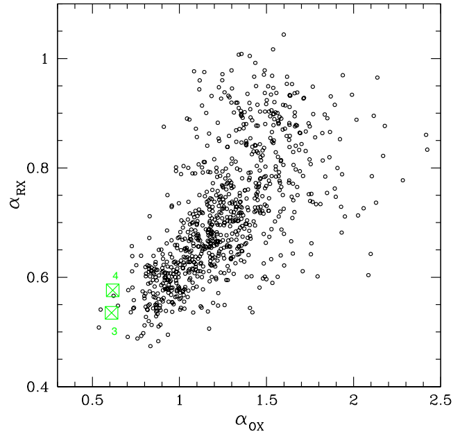
Figure 8. The \alpha_{OX}-\alpha_{RX} plane for the BL Lacs objects in the BZCAT catalogue (black open circle) and for the two EXO50 sources (open-crosses-green symbols) spectroscopically identified as BL Lacs reported in this paper.
