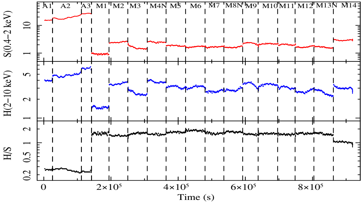
Fig. 1. Background subtracted XMM-Newton pn light curves of NGC 5548 calculated for the soft (S) 0.4–2 keV energy band (top), the hard (H) 2–10 keV energy band (middle) and their hardness ratios H/S (bottom). Vertical dashed lines indicate when observations were interrupted during the years.
