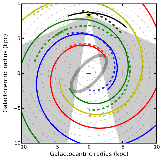
Figure 1. A bird's eye schematic of the Milky Way. The solid coloured spiral features correspond to the HH14 four-arm spiral arm model based on H II regions, where red is the Norma arm, yellow is the Perseus arm, green is the Sagittarius-Carina arm, blue is the Scutum-Centaurus arm, and black is the local arm. The grey ellipse represents the area influenced by the Galactic bar. The dashed lines show the Reid et al. (2016) loci of the spiral arms, colour-coded in kind as above. The star indicates the position of the Sun. The grey shaded regions show the area bound by the longitude limits of the current catalogue.
