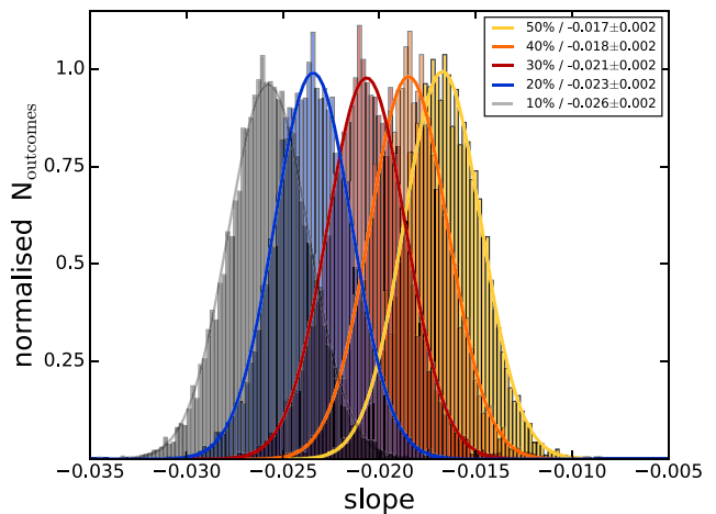
Figure 3. Distribution of slopes when randomly sampling ( N = 10\,000 times) within the distance estimation error. Different fractional errors are shown in the different colours: 50% (yellow), 40% (orange), 30% (red), 20% (blue) and 10% (grey). The key shows the mean and standard deviation of each distribution.
