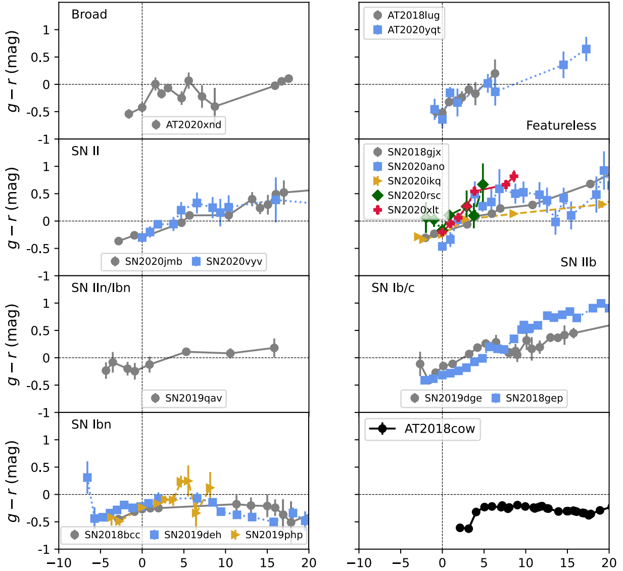
Figure 5. Color evolution of ZTF FBOTs, with AT2018cow shown on the lower right for comparison. Unlike AT2018cow, most events redden after peak, with the exception of the Type IIn SNe and potentially the radio-loud event AT 2020xnd.
