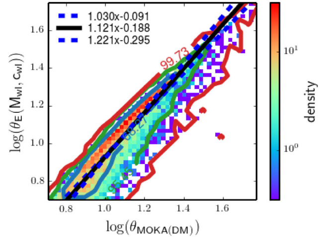
Figure 13. Scaling relation between the Einstein radius of an NFW halo with the same mass and concentration – computed by fitting with an NFW functional the weak lensing shear profile – and the size of the Einstein radius of the cluster. As in Fig. 12, we show the correlation only for the DM run and present in Table 3 the results for the runs with BCGs. Dashed blue lines show the least-squares fit to the data in the \log(\theta_E(M_{wl}, c_{wl})) - \log(\theta_E) and in the \log(\theta_E) - \log(\theta_E(M_{wl}, c_{wl})) spaces, while the black line displays the bisector of them.
