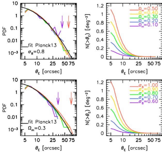
Figure 14. Left-hand panels: probability distribution functions of the Einstein radius distributions of a Monte Carlo realization of lenses at redshift z_l = 0.5 with sources located at z_s = 2.5 – the cluster number density has been computed from the Sheth & Tormen (1999) mass function integrated on the whole sky between z = 0.48 and 0.52 . Right-hand panels: cumulative number counts of strong lenses per square degrees with an Einstein radius larger than a fixed value. Top and bottom panels display the case of varying \Omega_M and \sigma_8 at a time, respectively. The black curve in the left-hand panels represents the lognormal relation (equation 17) that better describes the Planck13 probability distribution function. The arrows on the left-hand panels mark the largest Einstein radius find in the two extreme corresponding models.
