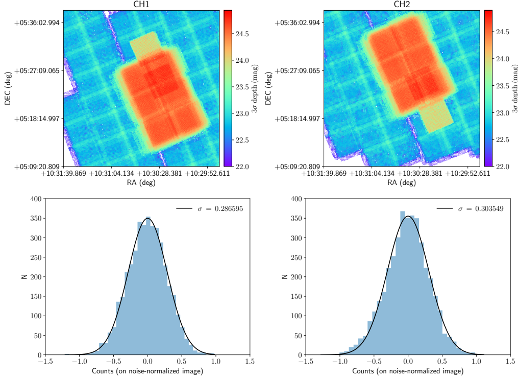
Figure 11. MUSYC1030: Top row: 3\sigma magnitude depths of 3.6\mu\text{m} and 4.5\mu\text{m} mosaics. Bottom row: Histograms of enclosed fluxes measured on \sim 4000 empty apertures in 3.6\mu\text{m} and 4.5\mu\text{m} on the noise-normalized images. Best-fit Gaussians are also shown.
