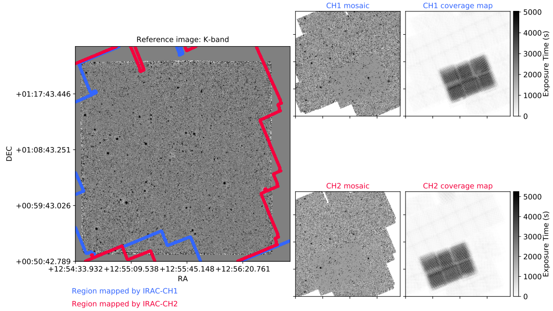
Figure 5. Same as in Figure 1, but for the MUSYC1255 field.
