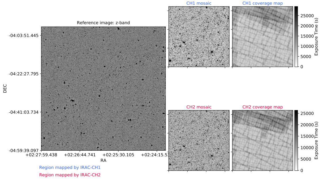
Figure 1. CFHTLS-D1: reference band mosaic, 3.6\mu\text{m} and 4.5\mu\text{m} mosaics and coverage maps. The coverage maps show where the individual pointings of IRAC overlap when they are combined to form the mosaic. Pixels with darker colors have more coverage.
