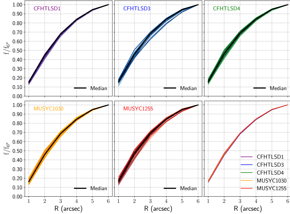
Figure 7. Same as in Fig. 6, but at 4.5\mu\text{m} .
