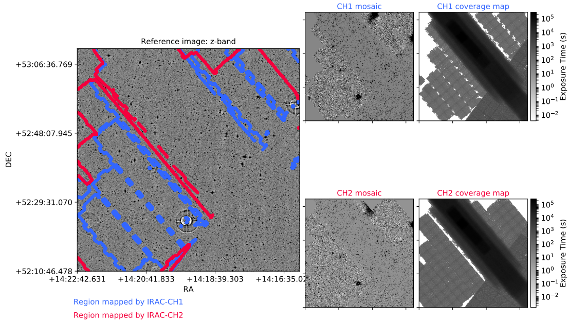
Figure 2. Same as in Figure 1, but for the CFHTLS-D3 field. For this field, we use a logarithmic scale for the coverage maps to show simultaneously the regions with the highest and lowest coverage.
