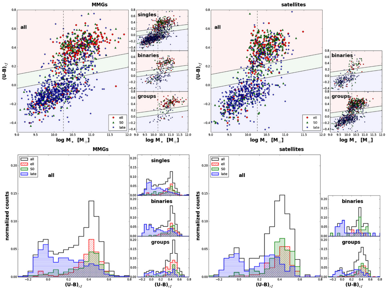
Figure 2. Rest-frame (U-B)_{rf} -mass relation (upper panels) and normalized rest-frame (U-B)_{rf} color distribution (bottom panels) for galaxies of different classes (left panels: MMGs, right panels: satellites) and morphologies in the different environments (shown in the smaller windows). Red circles and histograms: ellipticals; green triangles and histograms: S0s; blue stars and histograms: late types. In the upper panels, the black dashed vertical line represents the mass completeness limit, and the black solid lines show the separation between red, green, and blue galaxies (see the text for details).
