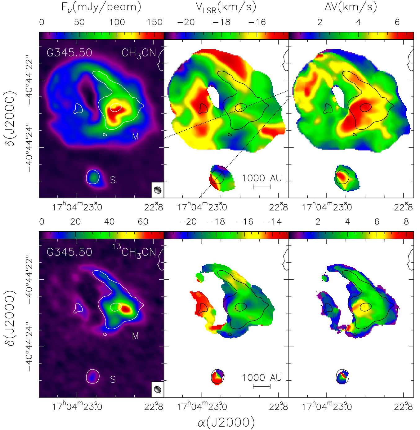
Fig. 11. Same as Fig. 7, but for G345.50. Labels M and S mark the corresponding cores, as in Fig. 2. The dotted lines denote the cuts adopted for the PV plots in Figs. 22 and 23.
