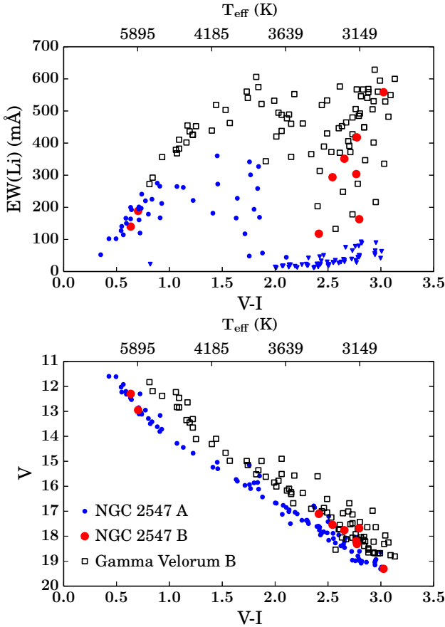
Fig. 3. Comparison between the multiple populations discovered in NGC 2547 and Gamma Vel B. The top panel shows the EW(Li) as a function of V - I , while the bottom panel shows a V vs. V - I CMD. Photometry has been corrected according to the extinction towards NGC 2547 ( E(B - V) = 0.06 ) and Gamma Velorum ( E(B - V) = 0.055 ). The x -axis on the top reports an effective temperature scale derived from V - I , using the colour-temperature transformations described in Pecaut & Mamajek (2013) . In both panels empty squares, filled red circles, and blue circles indicate the stars of Gamma Vel B, NGC 2547 B, and NGC 2547 A respectively. EW(Li) upper limits in NGC 2547 A are reported with downward triangles. Only a subsample of stars of NGC 2547 is shown, since V band photometry is not available for all targets (see footnote on page 4).
