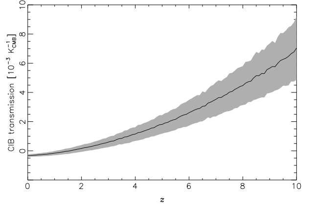
Figure 13. Predicted CIB transmission in the tSZ y-map for a hypothetical CIB emission of 1 \text{K}_{\text{CMB}} at 545 GHz and at redshift z . The shaded area represents the 68% confidence region, for uncertainties of \Delta T_d = 2 K and \Delta \beta_d = 0.1 in the modified blackbody parameters of the hypothetical CIB emission.
