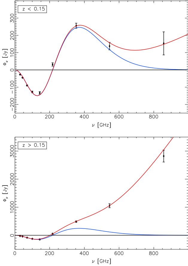
Figure 8. Observed SED of the stacked signal toward galaxy clusters, from 30 to 857 GHz. Top : objects below z = 0.15 . Bottom : objects above z = 0.15 . In blue we show the tSZ contribution to the total SED and in red the total SED considering infrared emission.
