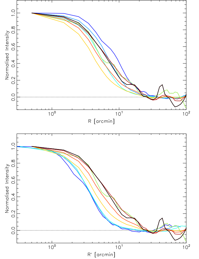
Figure 10. Top : observed radial profile of the stacked signal toward galaxy clusters at the native angular resolution at 70 GHz (in dark blue), 100 GHz (blue), 143 GHz (light blue), 217 GHz (green), 353 GHz (orange), 545 GHz (red), 857 GHz (dark red), and 100\mu\text{m} (black). Bottom : same as top panel, but as a function of the rescaled radius R' = R(\mathcal{B}_\nu/\mathcal{B}_{857}) .
