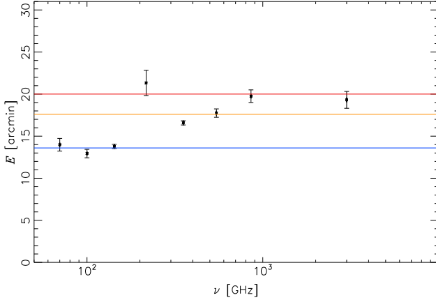
Figure 11. Variation of the spatial extension, \mathcal{E}(\nu) , of the stacked signal from 70 to 3000 GHz ( 100\mu\text{m} ). The blue line shows the expected value for the GNFW profile from Arnaud et al. (2010) and \theta_{500} values from PSZ1, the orange line shows the value we derive with the Xia et al. (2012) profile, and the red line shows the value for an NFW profile with c_{500} = 1.0 .
