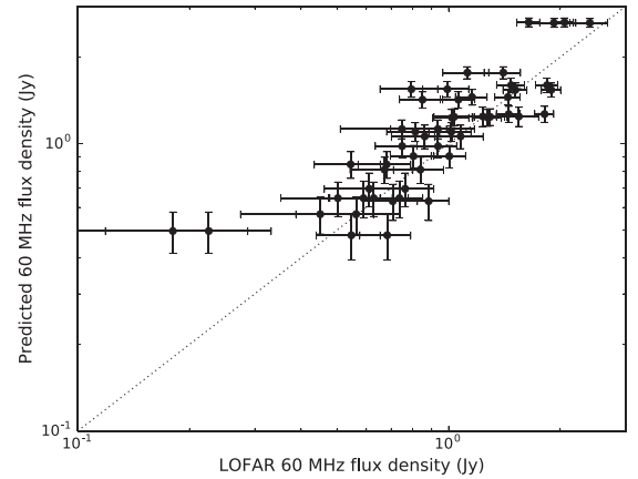
Figure 7. Flux comparison between LOFAR 60-MHz data and predicted 60-MHz fluxes from the VLSSr survey (assuming a spectral index of \alpha_{60}^{74} = -0.8 ). Only point sources are included due to the different resolution of the two surveys, but integrated flux densities are used to avoid the ionospheric smearing effects associated with the peak flux densities.
