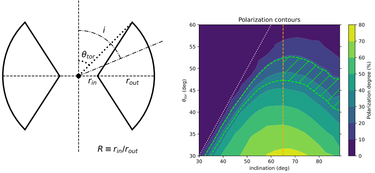
Figure 6. Left-hand panel: Sketch of the torus geometry assumed for polarimetric modelling. The torus opening angle \theta_{\text{tor}} and the observer inclination i are both measured from the symmetry axis. Right-hand panel: Contour plots of the constant polarization degree calculated for scattering off a torus, on the \theta_{\text{tor}} - i plane. The white dotted line corresponds to the equality \theta_{\text{tor}} = i ; the condition for the obscuration of the central source is \theta_{\text{tor}} < i . The green dashed curves enclose the 68 percent confidence level region on the measured polarization for the cold reflector in the Circinus galaxy. The orange dashed line marks the inclination of the host galaxy, likely a lower limit to the torus inclination (as discussed in the text). The green hatches mark the region of the parameter space consistent with all the observational constraints.
