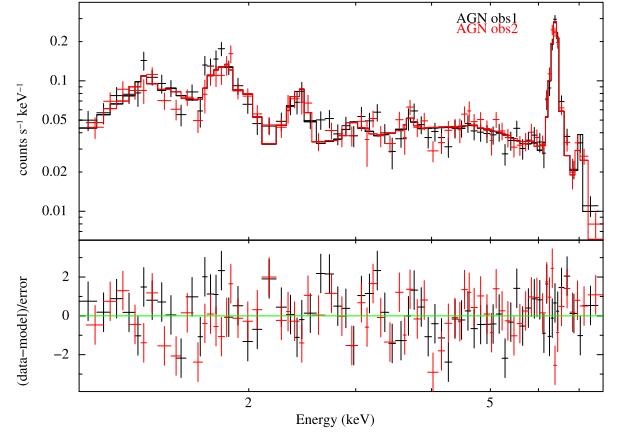
Figure A2. Chandra /ACIS spectra of the AGN with the best-fitting model in the 1–8 keV band. The black and red coloured crosses correspond to observation 1 and 2, respectively.
