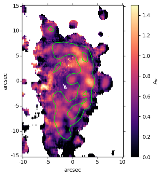
Figure 3. The V-band extinction map of the galaxy disc ( A_v in magnitude) derived from the Balmer decrement ( H\alpha/H\beta = 3.1 ) based on MUSE observations. The region near the centre where we are seeing reduced UV flux is not having a high extinction compared to the outer disc of the galaxy with enhanced UV flux. The green contour is taken from the NUV image shown in Fig. 2.
