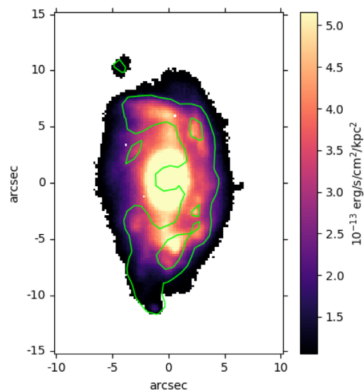
Figure 7. The MUSE image of the disc of JO201 created integrating 9050–9250 Å wavelength slice. The stellar bar like feature is clearly seen in the disc of galaxy. NUV contours are overlaid (in green) to highlight the cavity with reduced UV flux.
