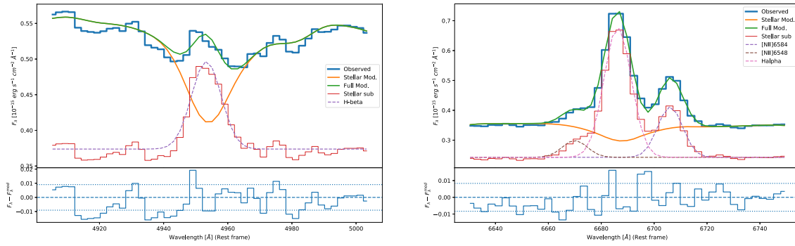
Figure A4. The 2021 GTC optical spectrum of 1ES 1927+654 zooming in the crucial H \beta and H \alpha regions. The stellar model and the emission-line fits are shown in the top panel of each of the two figures. The residuals compared to the full model, including the stellar model plus the emission-line fits, are plotted in the bottom panel. We do not detect any broad emission line in the 2021 spectra.
