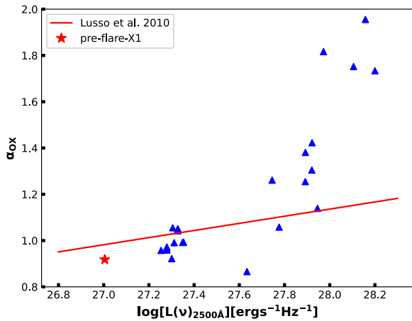
Figure 6. The \alpha_{OX} vs. L_{2500 \text{ \AA}} for the different Swift observations of the source IES 1927+654 as reported in Table 2. The red line denotes the best-fit correlation obtained from Lusso et al. (2010), which denotes the standard AGN disk–corona relation. The red star denotes the 2011 pre-CL state of IES 1927+654.
