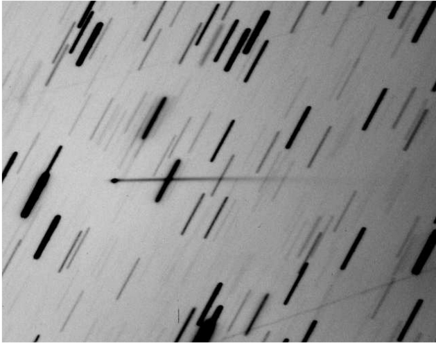
Figure 1. A 14 \times 11 arcmin picture of (6478) Gault with its tail taken from OAVdA on 2019 March 23, about 20:20 UT ( \alpha = 10^h 04^m 25.2^s , \delta = -01^\circ 08' 06''.7 ; J2000.0). North is up, east to the left. The main tail length is 5 arcmin 30 arcsec at position angle PA \approx 272^\circ . Its also visible a fainter 12 arcsec-extended antitail at PA \approx 91^\circ . The image is a stack of 38 frames, each with 180 s exposure time.
