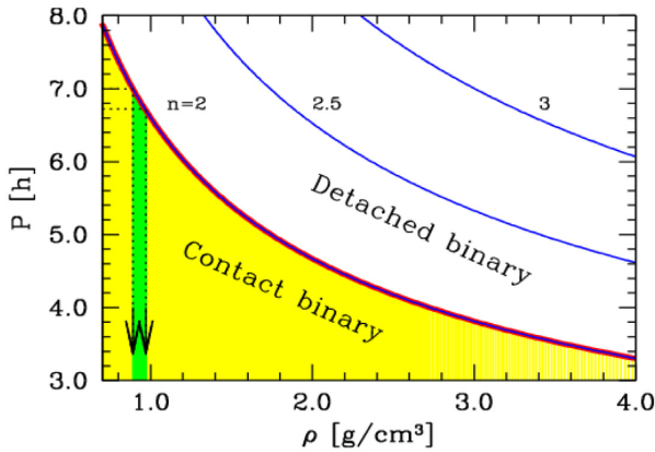
Figure 10. The expected P versus \rho relationship for a close binary system with the asteroid consisting of two components of similar size and mass, according to equation (7). The component distance is parametrized in terms of multiple ' n ' of the body's reference radius, R_G , as in equation (6). Accordingly, a contact system is obtained for n = 2 , while for n = 3 the two asteroid components are orbiting one R_G apart. The nominal periodicity of case P \approx 7 h is singled out in the plot, with an implied density for Gault of \rho \lesssim 1.0 \text{ g cm}^{-3} , in case of a contact binary system. The 6.7-h double periodicity, that occurred in MPO Canopus without using the March 30 Sanchez session, is also indicated. This gives an idea of the 'weight' that even a single session can have in these critical measures.
