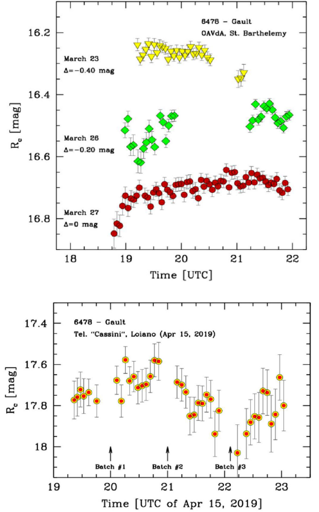
Figure 5. Gault’s observing sessions of 2019 March 23–27 from OAVdA (the mean uncertainty for the three sessions are, respectively, 0.020, 0.022, and 0.023 mag) and 2019 April 15 from Loiano (mean uncertainty 0.09 mag), are summarized in the upper and lower panels, respectively. The R_c magnitude scale is reproduced, throughout, from the local CMC-15 calibration, according to equation (4). Along the OAVdA observations, the asteroid was about its Earth opposition, at orbital phase angle \phi \sim 12.9^\circ , a figure that increased to \phi \sim 21.4^\circ for the Loiano data. The B, V magnitude sampling from Batch #1–3 observations is marked on the plot. Note a substantial difference in light-curve amplitude and shape between the two observing sessions. See text for a discussion.
