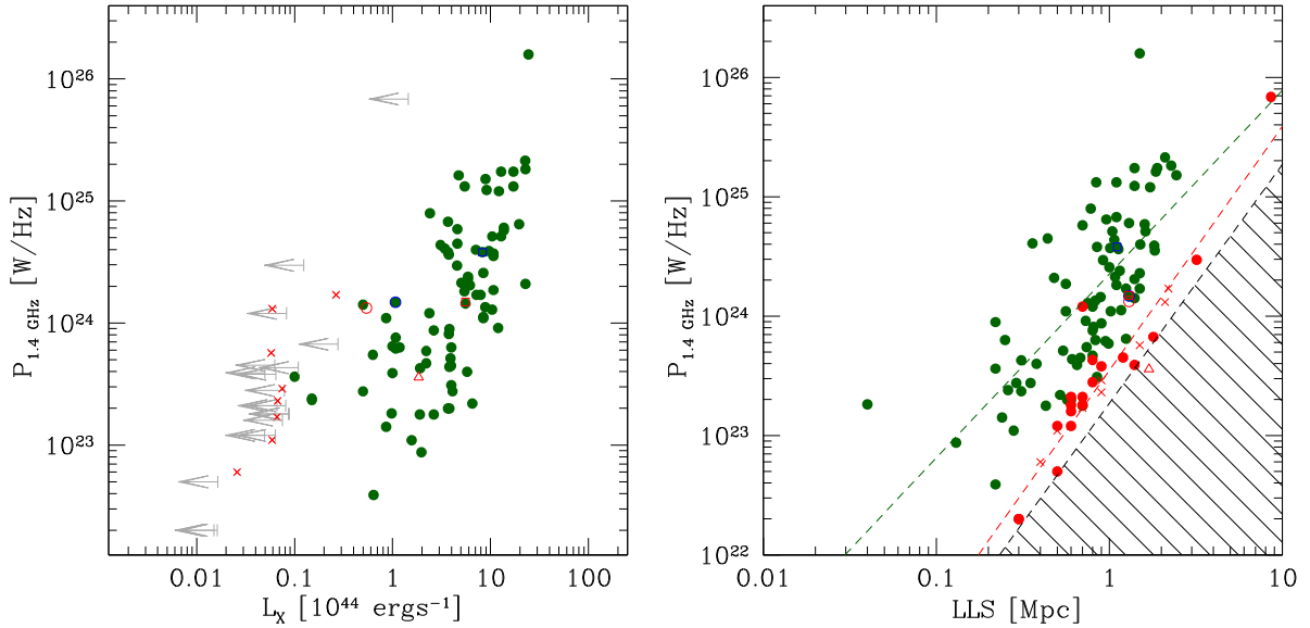
Figure 18. Left-hand panel: Radio power at 1.4 GHz P_{1.4 \text{ GHz}} versus X-ray luminosity in the energy band 0.1\text{--}2.4 \text{ keV} L_X , 0.1\text{--}2.4 \text{ keV} . Right-hand panel: Radio power P_{1.4 \text{ GHz}} versus LLS both at 1.4 GHz. Green dots and blue open symbols are from Feretti et al. (2012). Red symbols are measurements from this work: open symbols identify A523 (circle), A520 (square), G4 (triangle), while crosses identify the remaining sources with an X-ray identification. Grey arrows are upper limits from this work. The shaded area in the right-hand panel indicates the region of the (P_{1.4 \text{ GHz}}, \text{LLS}) plane that cannot be accessed considering the 2\sigma ( \sigma = 2.5 \text{ mJy beam}^{-1} ) sensitivity of the SRT+NVSS image after point-source subtraction. Dashed lines represent a linear fit in logarithmic scale of equation (1) for cluster sources (green) and for the new sources (red).
