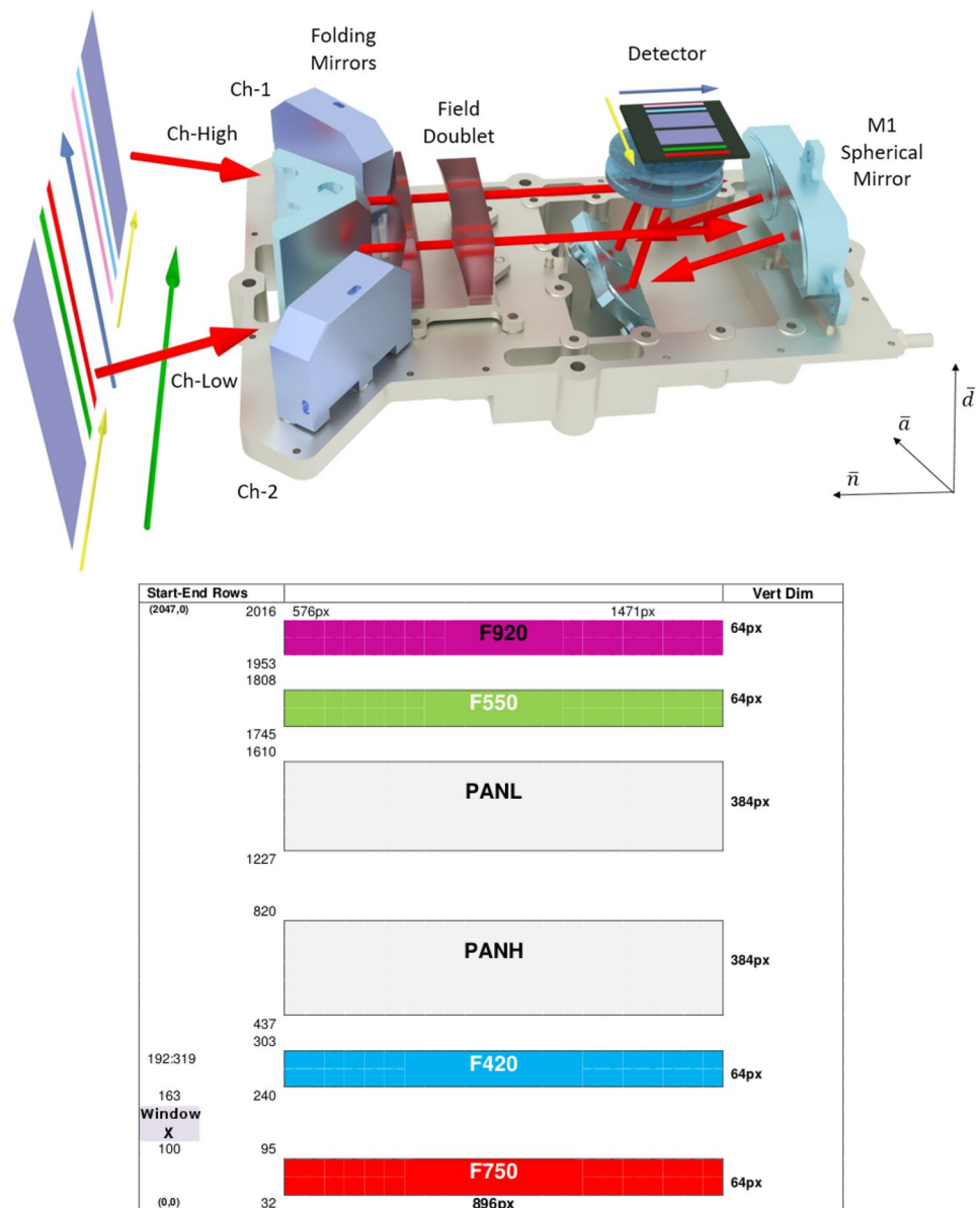
Fig. 1 STC optical scheme and detector configuration
