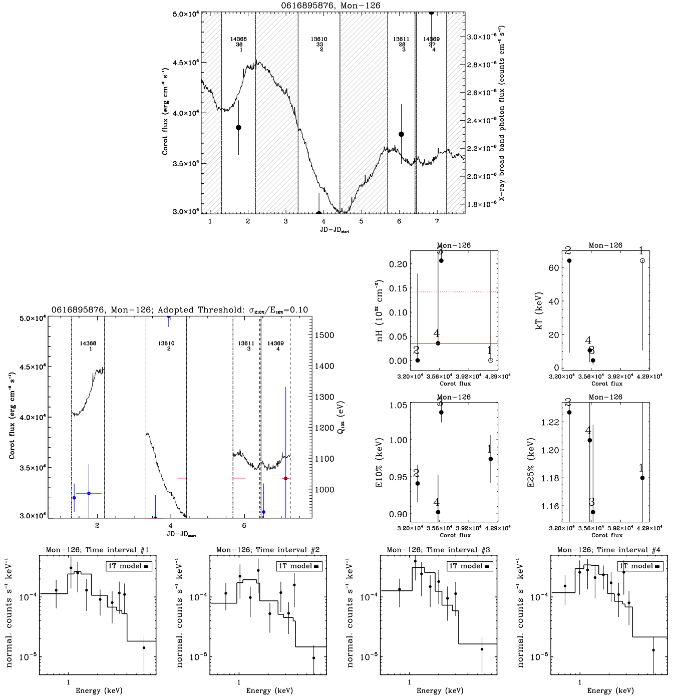
Fig. C.4. Variability and X-ray spectra of Mon-126, analyzed as a dipper. The CoRoT light curve shows dips without evidence of increasing N_H .
