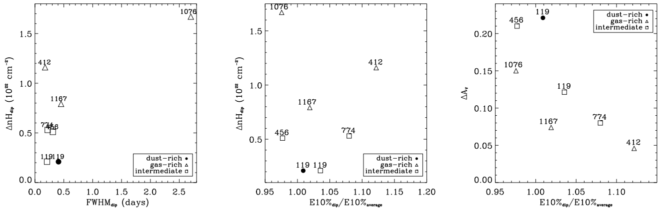
Fig. 23. Optical and X-ray properties of the dips where we observe an increasing X-ray absorption, described in Table 6. The left panel shows N_H versus FWHM of the dips, the central panel shows \Delta N_H due to the dips versus the ratio between the 10% photon energy quantile E_{10\%} observed during the dip and that in the average X-ray spectrum, and the right panel shows \Delta A_V increment observed during the dip versus the E_{10\% \text{ dip}}/E_{10\% \text{ average}} ratio. In all three panels , different symbols are used to mark dips with different N_H/A_V ratio and the labels show the stellar Mon-IDs.
