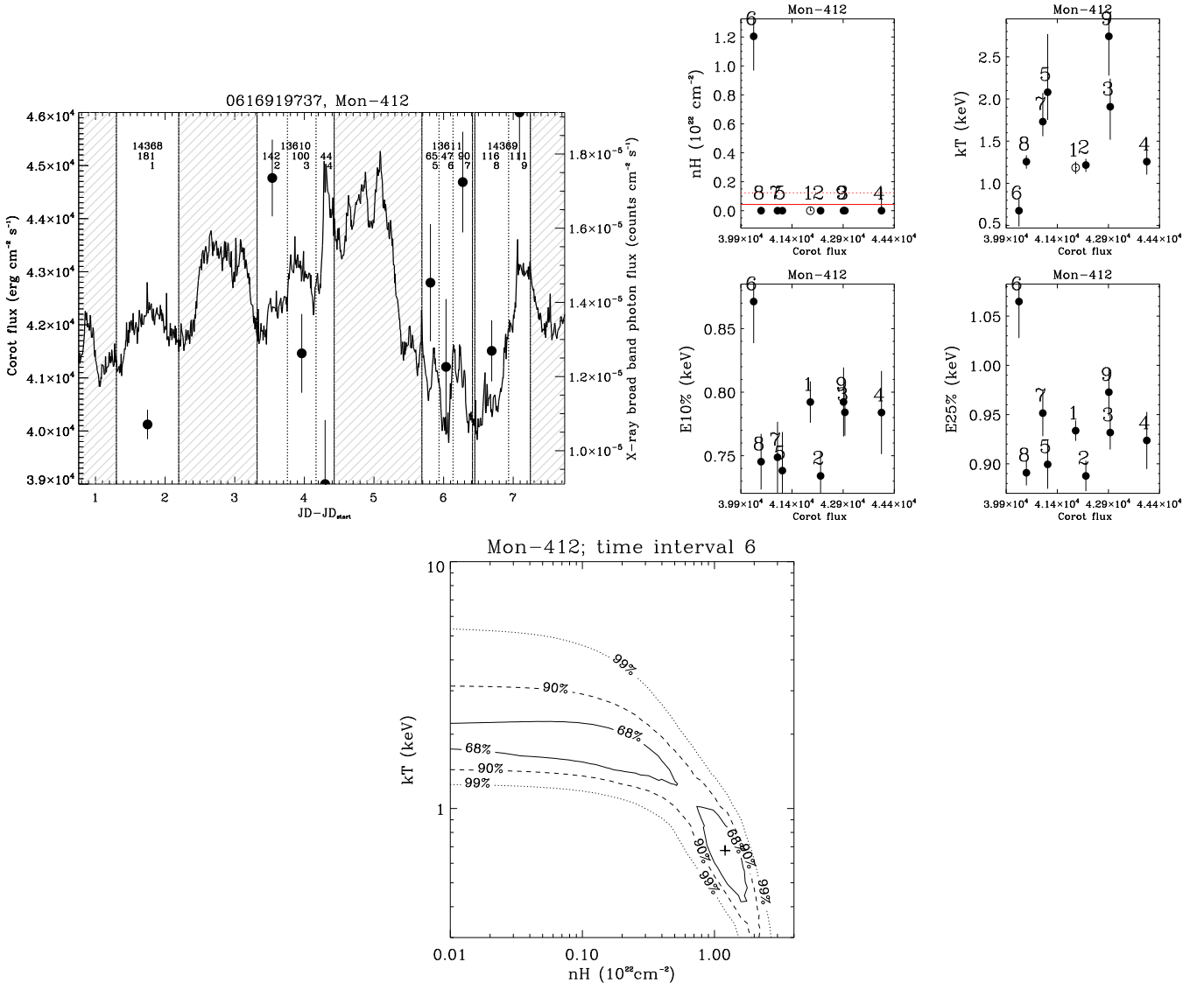
Fig. 6. Optical and X-ray variability of Mon-412. Panel format and content generally follows Fig. 4. In this case, we show the hydrogen column density N_{\text{H}} in units of 10^{22} cm -2 , the plasma temperature kT and the 10% and 25% photon energy quantiles in keV, and contour levels in the C-stat space. The contours are from the X-ray spectral fit of the spectrum observed during the interval #6.
