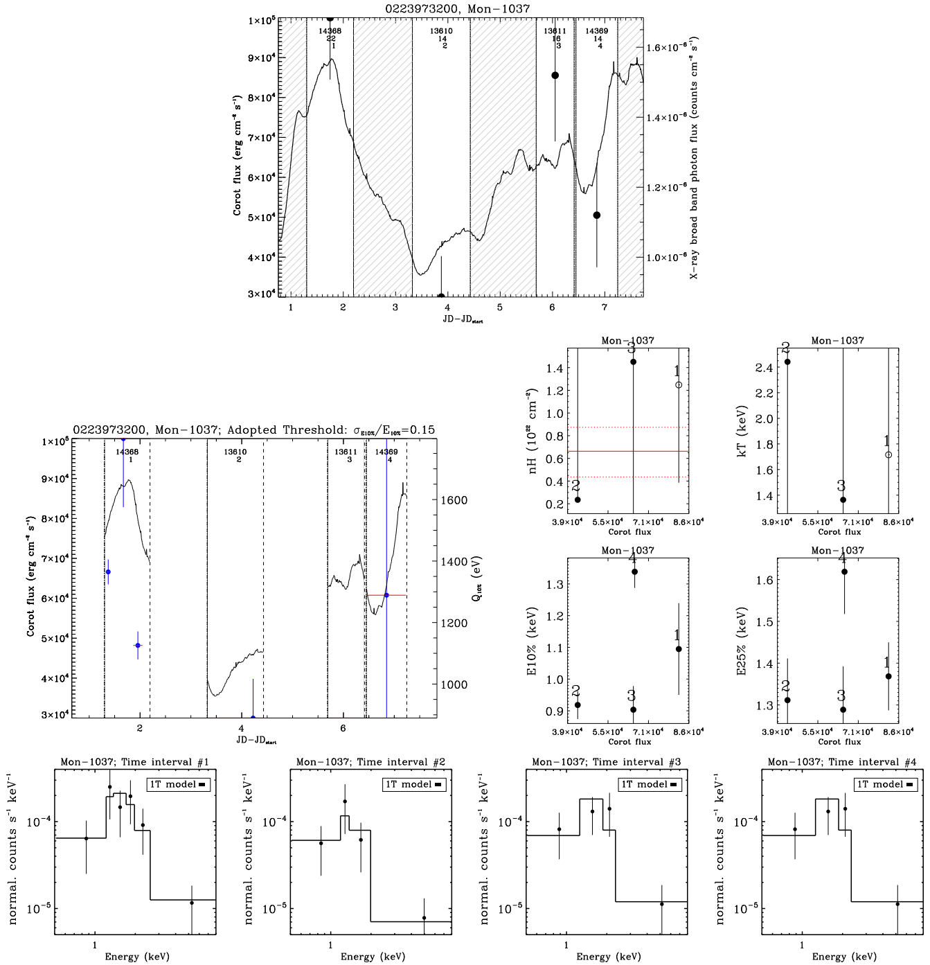
Fig. C.1. Variability and X-ray spectra of Mon-1037, analyzed as a dipper. E_{10\%} is larger during the dip in #4, but a significant variability of N_H is not observed.
