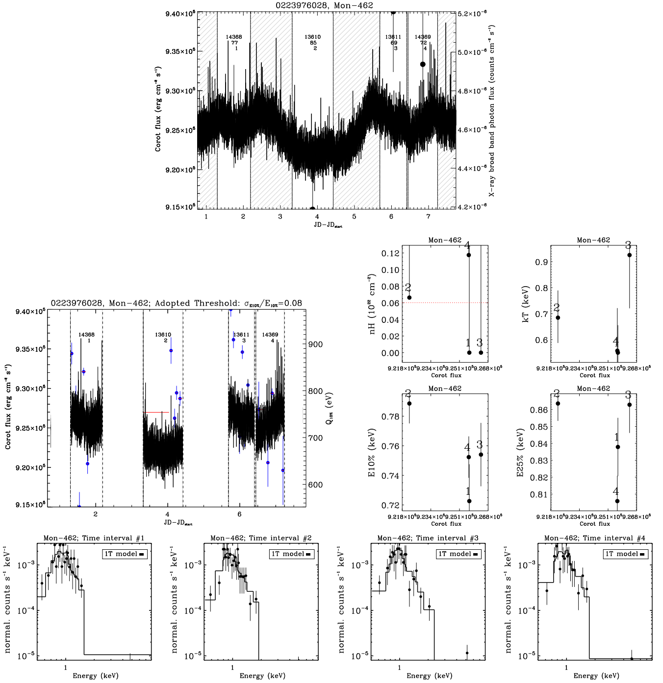
Fig. C.24. Variability and X-ray spectra of Mon-462, analyzed as a dipper, with a large optical dip observed, which however does not correspond to a significant increase of N_H .
