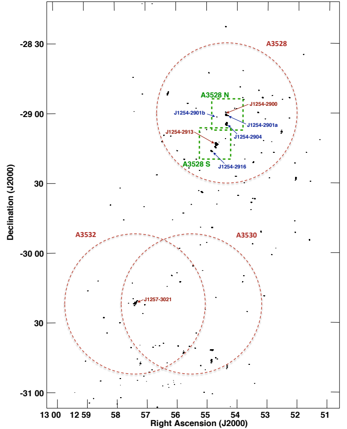
Fig. 1. Radio contours of the A 3528 complex at 610 MHz. The restoring beam is 6.8'' \times 4.7'' , PA 29^\circ and the noise level of 0.16 mJy beam ^{-1} . The levels are 7\sigma \times (1, 2, 4, 8, 16, 32, 128) . The dashed red circles show the Abell radius of the three clusters. The BCGs are labelled in red, the tailed radio galaxies in blue. The dashed green squares represent the A 3528 N and A 3528 S sub-clusters, based on the X-ray observations (Gastaldello et al. 2003).
