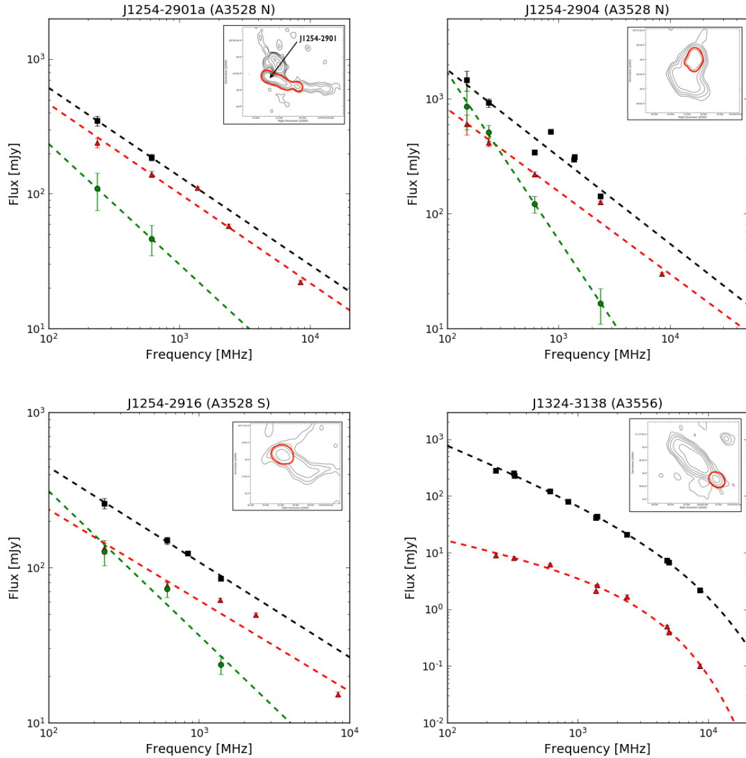
Fig. 7. Integrated radio spectra for the total (black) central (red), and diffuse (green) emission for the tails sample. The contours of the radio galaxy are displayed in the top right corner of each spectrum. The red line shows the region that has been taken as “central” emission.
