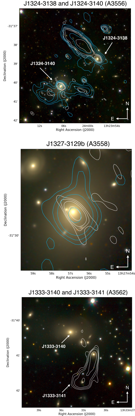
Fig. 5. VST-ACCESS gri composite images with GMRT radio contours at 325 (blue) and 610 (white) MHz. Top left panel: J1324-3138 and J1324-3140 (A3556). The 325 MHz contours are at 3\sigma \times (1, 2, 4, 8, 16) mJy beam ^{-1} , the resolution is 16.3'' \times 11.89'' , PA 12.29^\circ , and noise level \sigma_{325\text{ MHz}} = 0.20 mJy beam ^{-1} . The 610 MHz contours are at 3\sigma \times (2, 4, 8, 16) mJy beam ^{-1} , the resolution is 12.86'' \times 7.2'' , PA 41.78^\circ , and noise level \sigma_{610\text{ MHz}} = 0.08 mJy beam ^{-1} . Top right panel: J1327-3129b (A3558). The 325 MHz contours are at 3\sigma \times (2, 4, 8, 16) mJy beam ^{-1} , the resolution is 16.3'' \times 11.89'' , PA 12.29^\circ , and noise level \sigma_{325\text{ MHz}} = 0.25 mJy beam ^{-1} . The 610 MHz contours are at 3\sigma \times (2, 4, 8, 16) mJy beam ^{-1} , the resolution is 10.98'' \times 5.59'' , PA 34.16^\circ , and noise level \sigma_{610\text{ MHz}} = 0.14 mJy beam ^{-1} . Bottom panel: J1333-3140 and J1333-3141 (A3562). The 610 MHz contours are at 3\sigma \times (2, 4, 8, 16) mJy beam ^{-1} , the resolution is 8'' \times 6'' , PA 0^\circ , and noise level \sigma_{610\text{ MHz}} = 0.08 mJy beam ^{-1} .
