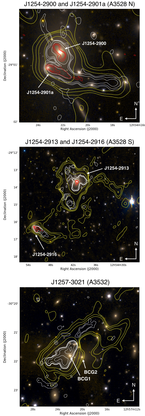
Fig. 3. VST-ACCESS gri composite images with GMRT radio contours at 235 (yellow) and 610 (white) MHz and VLA radio contours at 8.4 GHz (red). Top left panel: J 1254-2900 and J 1254-2901a (A 3528 N). Top right panel: J 1254-2913 and J 1254-2916 (A 3528 S). The 235 MHz contours are at 3\sigma \times (1, 2, 4, 8, 16) mJy beam ^{-1} , the resolution is 16.3'' \times 11.9'' , PA 9.5^\circ , and noise level \sigma_{235\text{ MHz}} = 1.26 mJy beam ^{-1} . The 610 MHz contours are at 3\sigma \times (1, 2, 4, 8, 16) mJy beam ^{-1} , the resolution is 6.8'' \times 4.7'' , PA 29^\circ , and noise level \sigma_{610\text{ MHz}} = 0.21 mJy beam ^{-1} . The 8.4 GHz contours are at 3\sigma \times (1, 4, 8) mJy beam ^{-1} , the resolution is 2.76'' \times 1.59'' , PA 49.82^\circ , and noise level \sigma_{8.4\text{ GHz}} = 0.05 mJy beam ^{-1} . Bottom panel: J 1257-3021 (A 3532). The 235 MHz contours are at 3\sigma \times (1, 2, 4, 8, 16) mJy beam ^{-1} , the resolution is 16.3'' \times 11.9'' , PA 9.5^\circ , and noise level \sigma_{235\text{ MHz}} = 0.76 mJy beam ^{-1} . The 610 MHz contours are at 3\sigma \times (1, 2, 4, 8, 16, \dots) mJy beam ^{-1} , the resolution is 6.8'' \times 4.7'' , PA 29^\circ , and noise level \sigma_{610\text{ MHz}} = 0.14 mJy beam ^{-1} .
