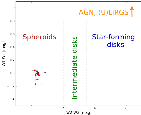
Fig. 9. Position of the 12 radio galaxies (dots with error bars) in the WISE colour-colour diagram. The diagram is divided into regions of colours characterizing different galaxy types following Jarrett et al. (2017; cf. their Fig. 11).
