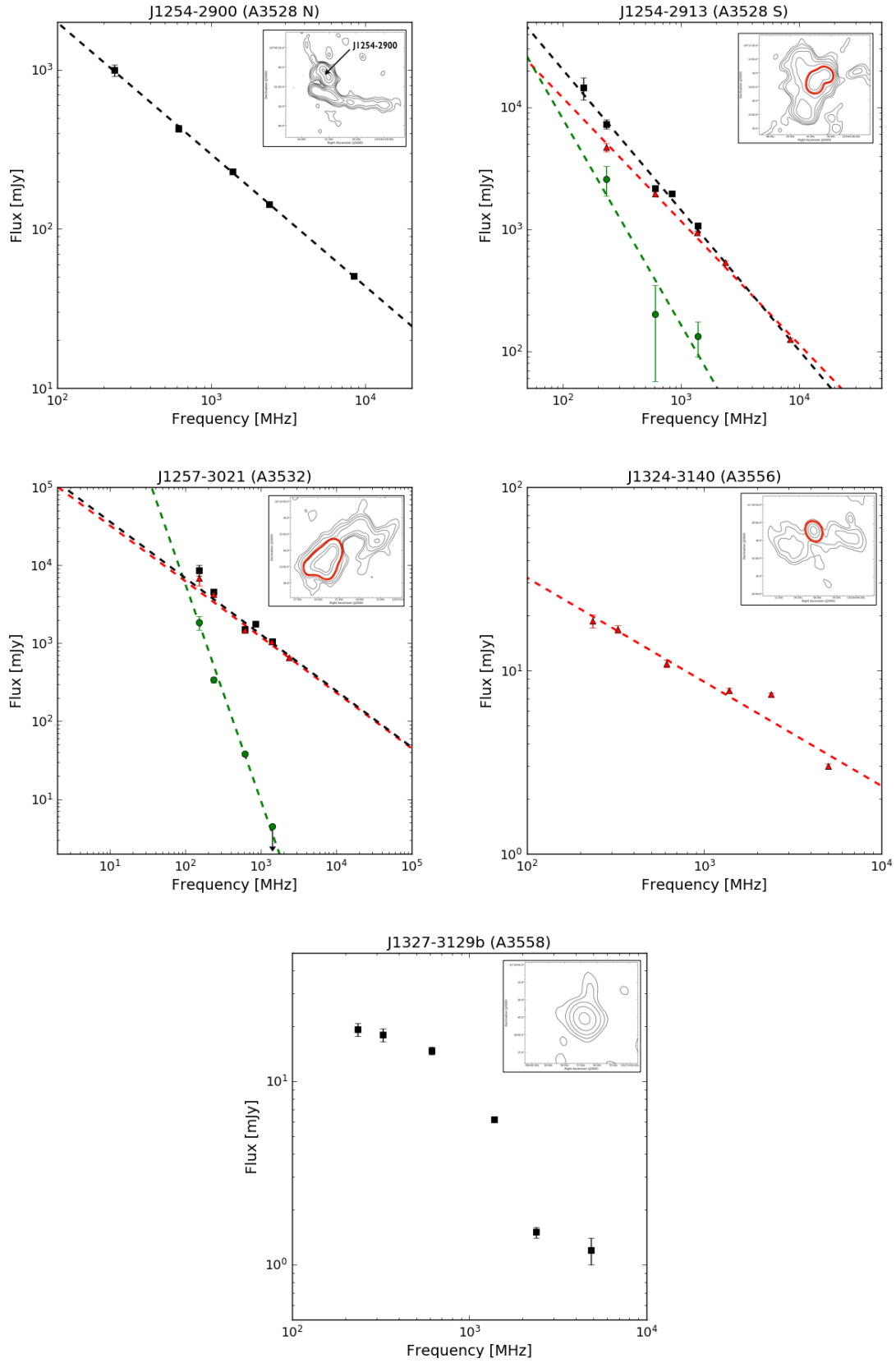
Fig. 6. Integrated radio spectra for the total (black) central (red), and diffuse (green) emission for the BCGs sample. The contours of the radio galaxy are displayed in the top right corner of each panel. The red line shows the region that has been taken as “central” emission. The value at 1.4 GHz in the J 1257-3021 (A 3532) spectrum is an upper limit.
