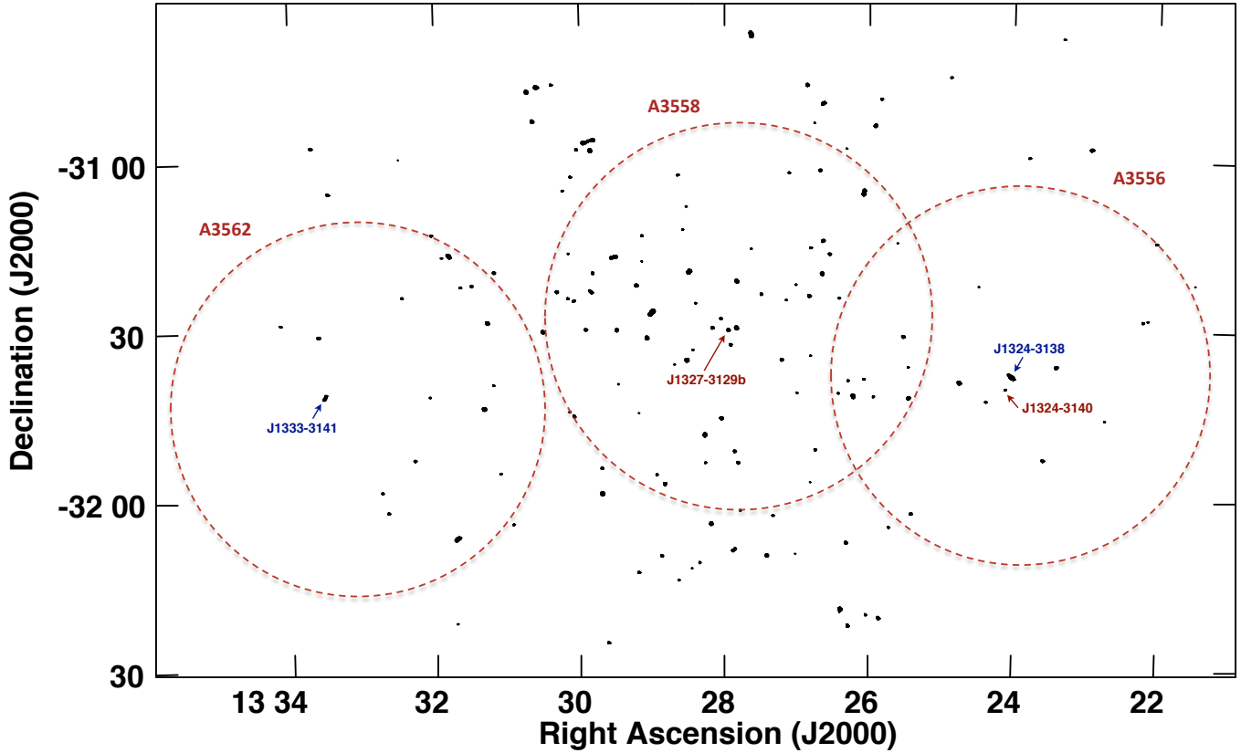
Fig. 2. Radio contours of the A 3558 complex at 325 MHz. The restoring beam is 14.05'' \times 9.53'' , PA equal to 18.39^\circ and the noise level of 0.09 \text{ mJy beam}^{-1} . The levels are 7\sigma \times (1, 2, 4, 8, 16, 32, 128) . The dashed red circles show the Abell radius of the three clusters. The BCGs are labelled in red, the tailed radio galaxies in blue.
