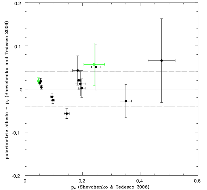
Figure 4. Plot of the difference between the albedo values derived using the new calibration coefficients of the slope–albedo relation for objects included in the Shevchenko & Tedesco (2006) list and the corresponding values found by the above authors. The dashed lines correspond to differences of \pm 0.04 in albedo. The meaning of the symbols is the same as in Fig. 2.
