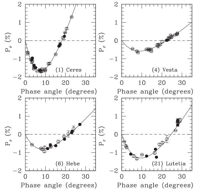
Figure 1. Examples of phase–polarization curves obtained for four large main belt asteroids belonging to different taxonomic classes: top left: the dwarf planet (1) Ceres (G-class); top right: (4) Vesta (V-class); bottom left: (6) Hebe (S-class); bottom right: (21) Lutetia (for a long time considered to belong to the old M class, now included in the X complex). Open symbols refer to data available in the literature. Full symbols in the plots identify observations obtained at the CASLEO observatory. Most of them have been published only recently (Gil Hutton et al. 2014). The best-fitting lines correspond to the exponential–linear relation discussed in Section 5.
