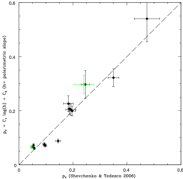
Figure 3. Comparison between the albedos of 15 objects observed in our campaign, derived using our new calibration coefficients of the slope–albedo relation, and the corresponding albedo values given by Shevchenko & Tedesco (2006). The meaning of the symbols is the same as in Fig. 2
