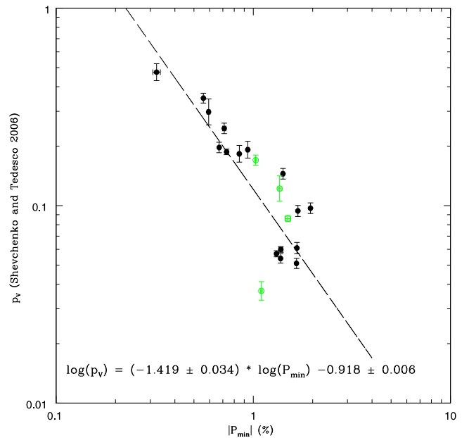
Figure 11. Best-fitting relation between P_{\min} and geometric albedo for an available sample of 20 asteroid targets included in the Shevchenko & Tedesco (2006) list. Only 16 objects for which we have at disposal at least 10 polarimetric measurements have been used to derive the best-fitting solution. These objects are plotted as full, black symbols. Open, green symbols represent objects for which we have fewer than 10 observations, and were not used in the least-squares computation.
