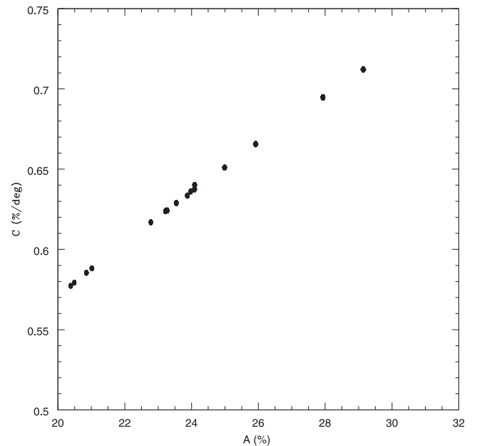
Figure 10. The same as in Fig. 9, but for the A and C parameters in equation (4).
