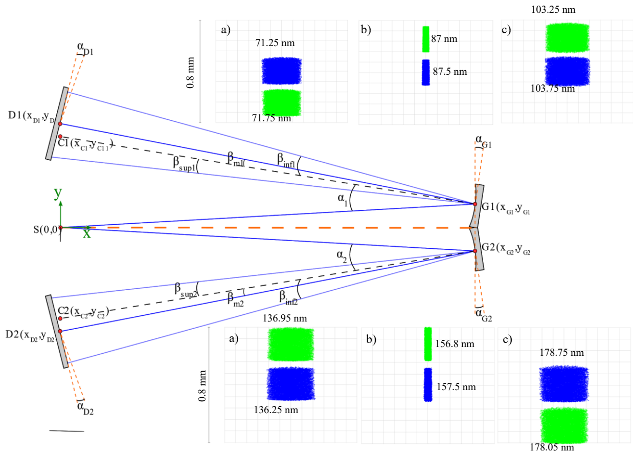
Fig.1 Dual channel optical design and simulations.
