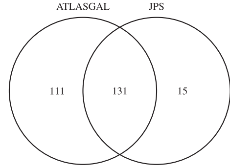
Figure 4. Venn diagram presenting the matching statistics for detected masers in the region \ell = 20^\circ – 60^\circ . The total sample of methanol masers in this region is 265, for which we have found a match to either ATLASGAL or JPS for 257 of these. Manual extraction has been used for 10 of the ATLASGAL matches and 4 of the JPS matches. For the six sources with no corresponding detection in ATLASGAL and for a further eight sources where JPS better describes the clump distribution, we have opted to use the JPS flux values.
