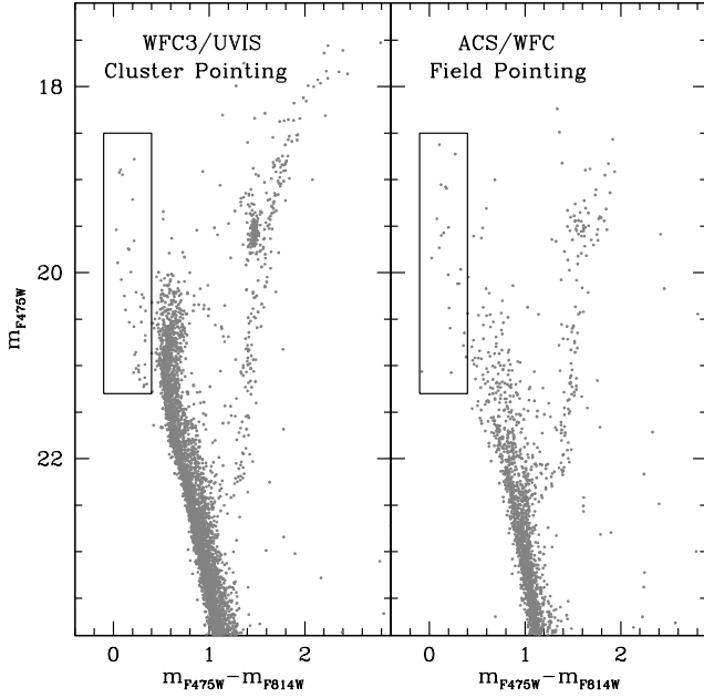
Fig. 2. ( m_{\text{F475W}} , m_{\text{F475W}} - m_{\text{F814W}} ) CMDs of the Cluster Pointing and Field Pointing . The black boxes highlight the BSS region that has been used in the analysis (see Sect. 3).
