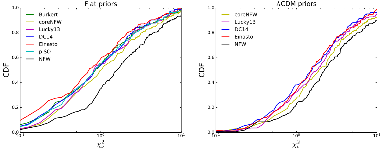
Figure 1. Cumulative distributions of the reduced \chi^2_\nu for seven halo profiles with flat (left) and \Lambda CDM priors (right).
