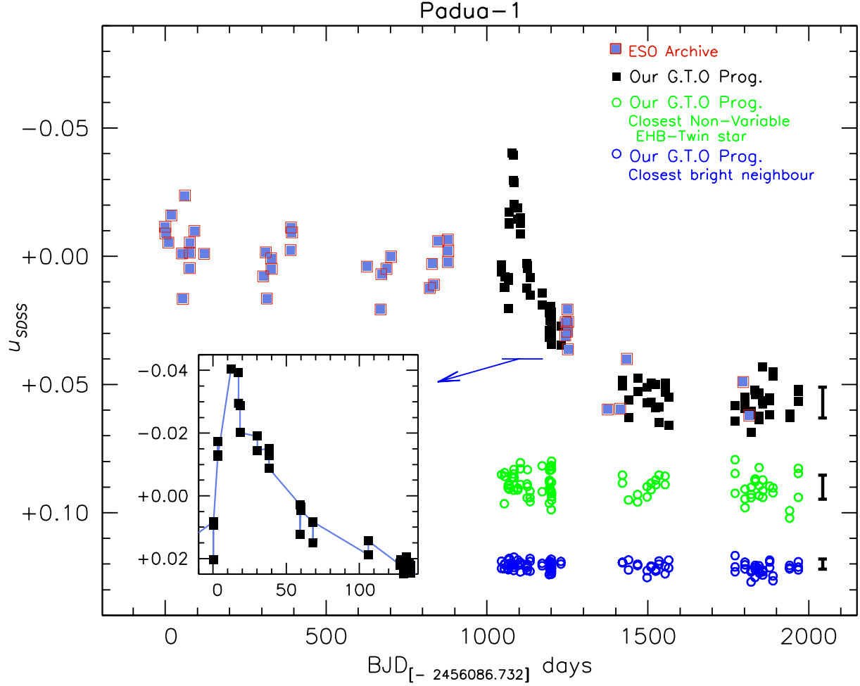
Figure 4: The u_{SDSS} light curve of the EHB Padua-1 showing a complete superflare event. Light blue squares display the six-year monitoring of Padua-1 using archival OmegaCAM@VST data, while black squares display our three-year monitoring using the same instrument/filters/exposure times but collected with better seeing and more frequent sampling. The agreement between the two data-sets is evident. Two comparison stars (green/blue open circles) along with their respective 1 - \sigma photometric error bars are also plotted. The constant trends displayed by the comparison stars (at only \sim 20'' and \sim 13'' from Padua-1) prove that the \sim 0.05 mag fainting and the \sim 80 -day superflare event are intrinsic to Padua-1.
