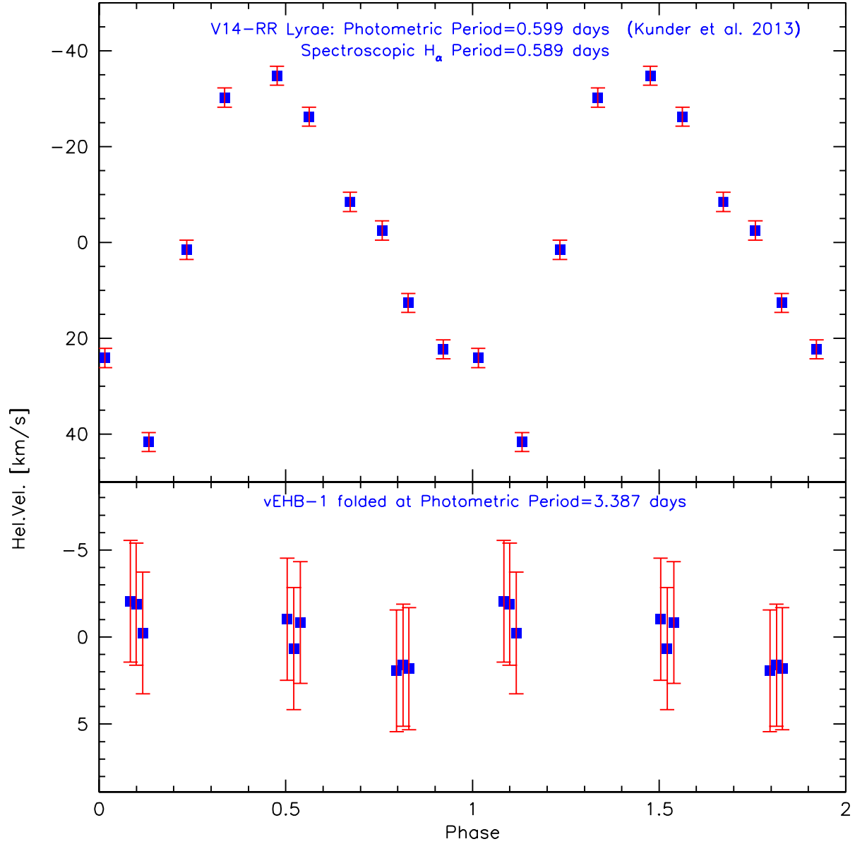
Supplementary Figure 2: No binarity signature detected in the NGC2808 vEHB-1 variable. Upper panel displays the phased H_{\alpha} radial velocity curve of a comparison RR Lyrae proving a successful detection of velocity variations in the data-set. The lower panel displays the velocity curve of our photometric variable vEHB-1 present in the same data-set. The error bars display the 1 - \sigma error ( \sim 3.5 km/s) estimated at the vEHB-1 luminosity. No significant velocity variations for vEHB-1 are observed. For clarity, the NGC2808 average radial velocity has been subtracted.
