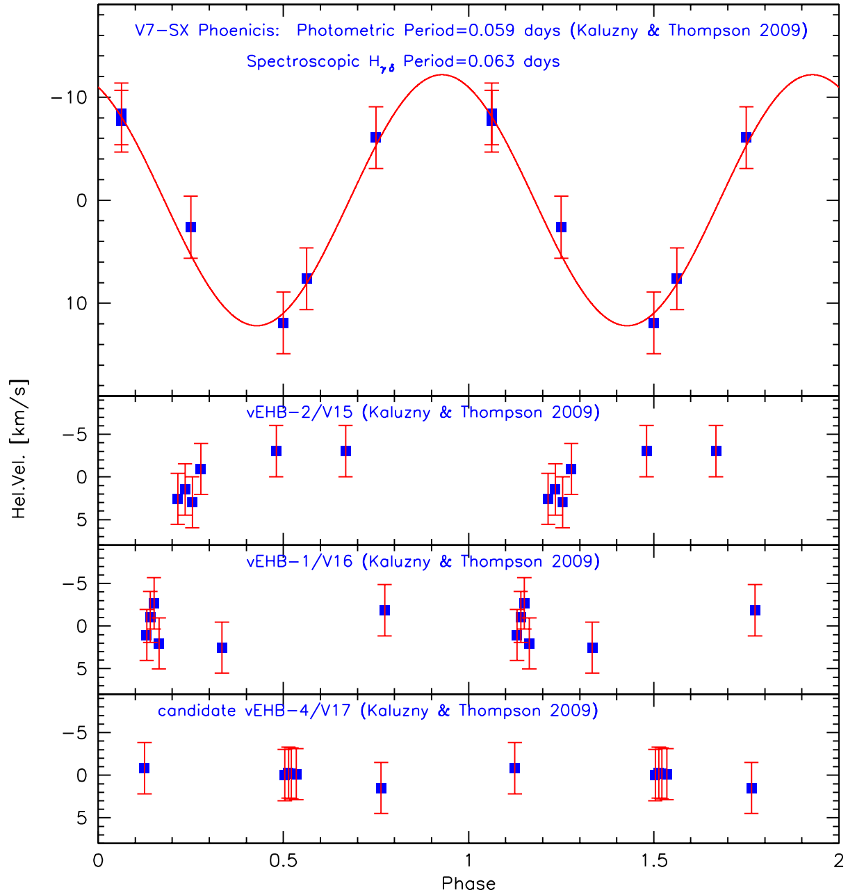
Supplementary Figure 3: No binarity signature detected in the NGC6752 vEHB-1/2 variables. Upper panel displays the phased H_{\gamma\delta} radial velocity curve of a comparison SX Phoenixis star 46 proving a successful detection of velocity variations in the data-set. The lower panels display the velocity curves of the 2 EHB photometric variables (and the candidate EHB photometric 46 variable vEHB-4/V17) present in the same data-set. The error bars display the 1 - \sigma error ( \sim 3.0 km/s) estimated at the vEHB-1 luminosity. No significant velocity variations for the vEHB-1/2 are observed. For clarity, the NGC6752 average radial velocity has been subtracted.
