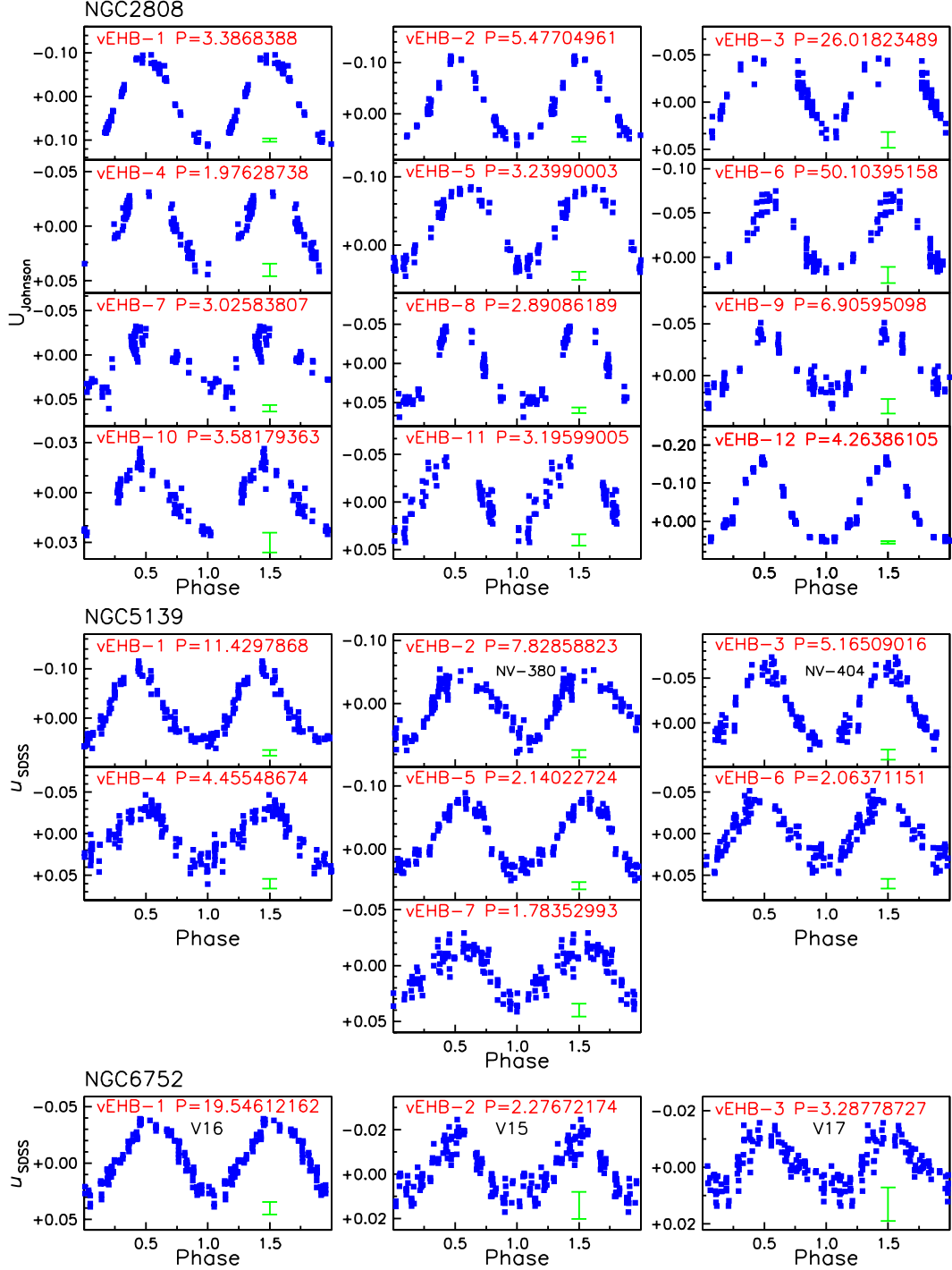
Figure 1: The phased near-ultraviolet light curves of the EHB variables in three globular clusters. The phased epochs are repeated twice for a better display of the periodicity. We used the U_{\text{Johnson}} -filter for the NGC2808 data (collected with VIMOS at the UT3 telescope) and the u_{\text{SDSS}} -filter for the NGC6752 and NGC5139 data (collected with OmegaCAM at the VST telescope). For each variable we report an assigned-identifier, the photometric period in days, and the typical 1 - \sigma photometric uncertainty of the measurements (plotted as an error bar).
