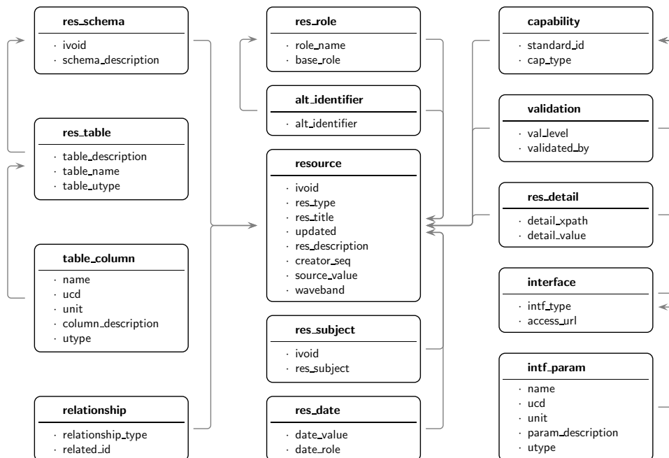
Figure 2: A sketch of the Relational Registry schema. Only the columns considered most interesting for client use are shown. Arrows indicate foreign key-like relationships.
