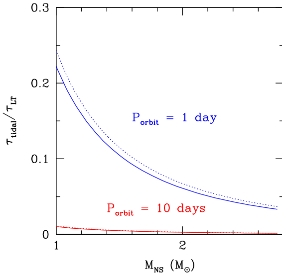
Figure 7. The ratio of the respective tidal to Lense-Thirring torques assuming a mass for the secondary star in the range of 18 (solid line)–23 (dotted line) M_{\odot} (Motch et al. 2014) and an orbital period consistent with observations of supergiant HMXBs (i.e. of order days; e.g. Corbett & Krimm 2013). While we have assumed B = 1 \times 10^{12} G, we note that the torque ratio decreases with decreasing field strength. Clearly the Lense-Thirring torque is expected to dominate the flow.
