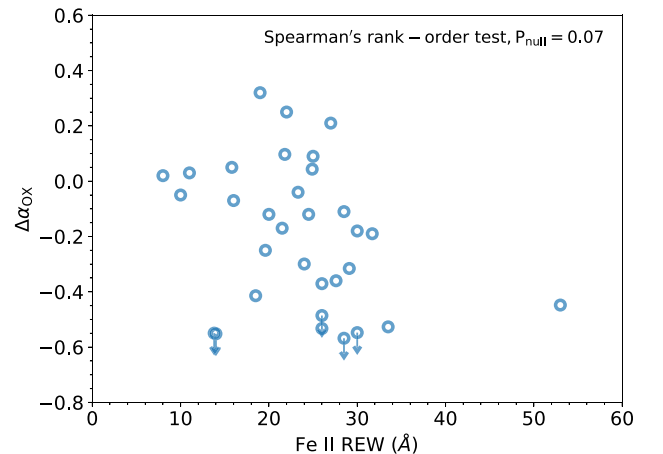
Figure 6. \Delta\alpha_{\text{OX}} versus Fe II REW for WLQs in the representative sample. For X-ray non-detections, the 90 per cent confidence upper limits of \Delta\alpha_{\text{OX}} are marked as the downward arrows.
