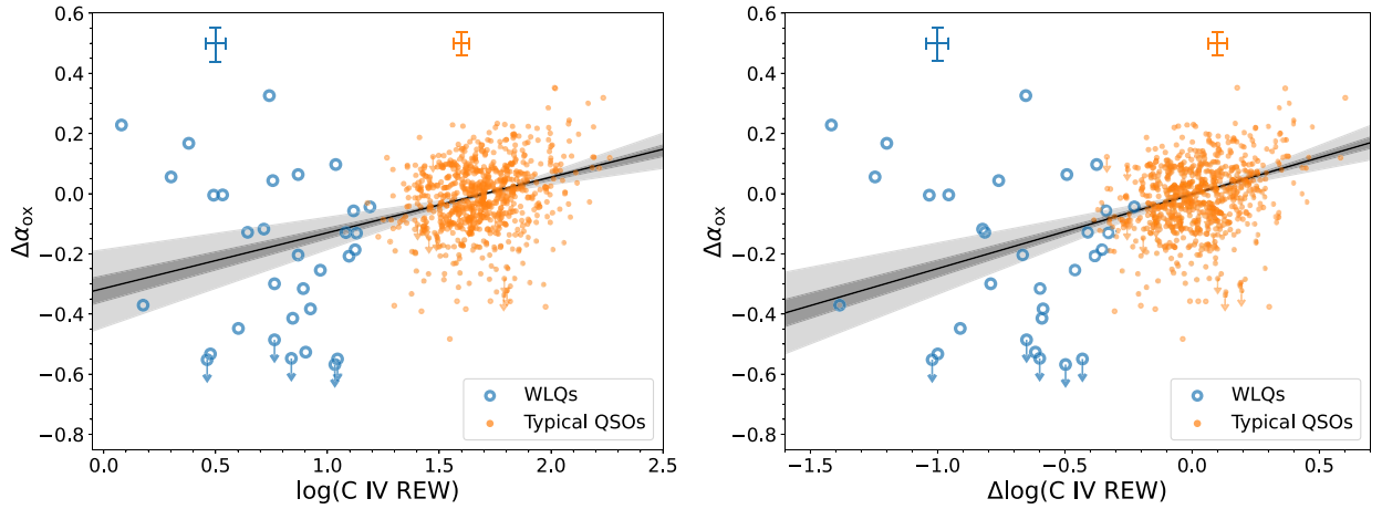
Figure 3. Left: \Delta\alpha_{\text{ox}} versus \log \text{C IV REW} (in units of \text{\AA} ) for WLQs in the representative sample as well as typical quasars in Timlin et al. (2020a). Right: \Delta\alpha_{\text{ox}} versus \Delta\log \text{C IV REW} for WLQs in the representative sample as well as typical quasars in Timlin et al. (2020a). The best-fitting \Delta\alpha_{\text{ox}}-\text{C IV REW} ( \Delta\alpha_{\text{ox}}-\Delta\log \text{C IV REW} ) relation (Timlin et al. 2020a) is shown as the black solid line, with its 1\sigma/3\sigma confidence intervals shown as the dark/light grey-shaded region in the left (right)-hand panel. The median measurement errors of \Delta\alpha_{\text{ox}} and C IV REW for WLQs and typical quasars are shown as error bars at the top of each panel.
