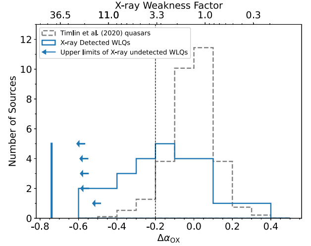
Figure 2. Distribution of \Delta\alpha_{\text{ox}} values. The solid histogram represents the \Delta\alpha_{\text{ox}} distribution of the 27 WLQs in the representative sample that are X-ray detected. The leftward arrows show the 90 per cent confidence \Delta\alpha_{\text{ox}} upper limits for five X-ray non-detected WLQs. The vertical bar represents the stacked \Delta\alpha_{\text{ox}} upper limit for these X-ray non-detected WLQs. The dashed histogram represents the \Delta\alpha_{\text{ox}} distribution for the Timlin et al. (2020a) quasar sample that has a \approx 99.3 per cent detection fraction, which is plotted for comparison (scaled to have the same apparent number of sources as the WLQ sample). The vertical dashed line (at \Delta\alpha_{\text{ox}} = -0.2 ) represents the adopted threshold for defining X-ray weakness in this study.
