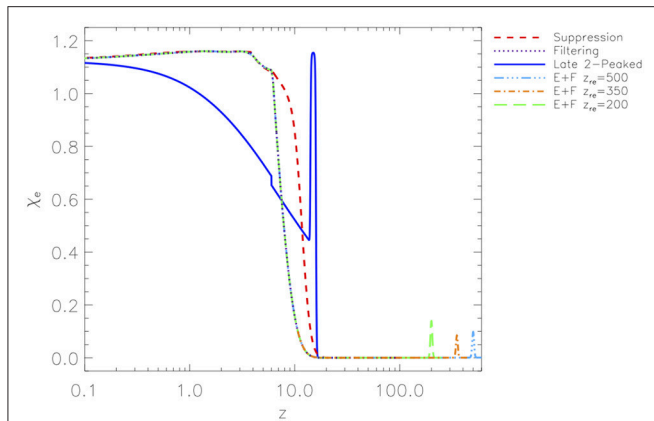
FIGURE 1 | Redshift dependence of the electron ionization fraction for a set of astrophysical and phenomenological reionization histories. For the considered phenomenological models the lower contribution to the global value of \tau at z < 10 is compensated by a peaked ionization phase at higher redshift. See also the text. Reprinted from Trombetti and Burigana (2012).
