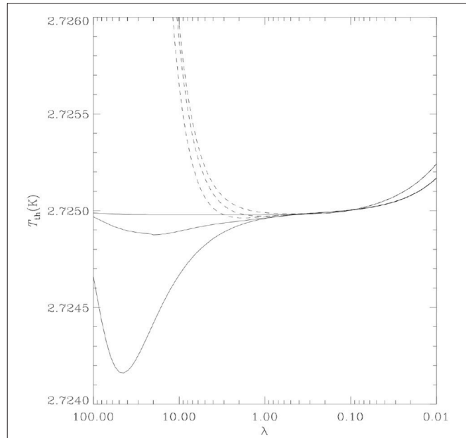
FIGURE 4 | “Distorted spectra in equivalent thermodynamic temperature vs. \lambda (in cm) with late energy injection \Delta\epsilon/\epsilon_i \simeq 4y = 5 \times 10^{-6} plus an early/intermediate energy injection \Delta\epsilon/\epsilon_i = 5 \times 10^{-6} ( \sim 20 times smaller than current upper limits) at the “time” Comptonization parameter y_h = 5, 1, 0.01 (bottom to top; the cases at y_h = 5 and 1 are very similar at short \lambda ; solid lines) plus a FF distortion with y_B = 10^{-6} (dashes).” y_h = y , but assuming electron temperature equal to the radiation one and computing the integral “from the energy injection time to the current time.” For a negative value of distortion parameter the shape of the distorted spectrum is almost specular with respect to a horizontal line with T = T_0 to that derived assuming the same absolute, but positive, parameter value. Reprinted from Burigana et al. (2004), Copyright (2004), with permission from Elsevier.
