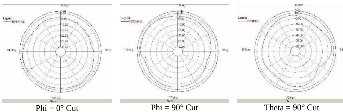
Figure 4.11: 2D Gain Radiation Patterns (principal cuts) @ 1575 MHz of hp iPAQ.
