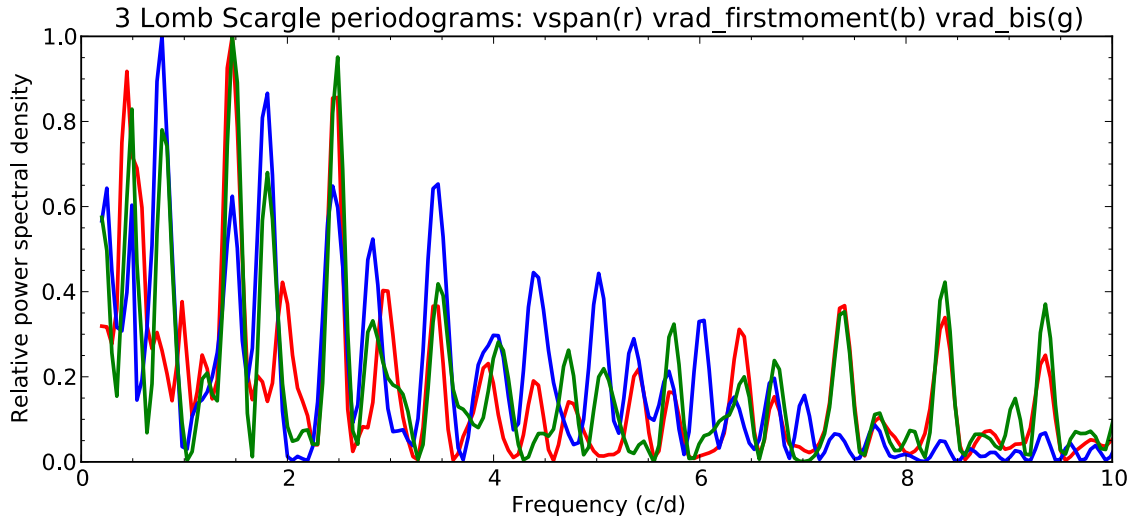
Fig. 16. Lomb Scargle periodogram showing the frequencies present in vspan (red), vrad (first moment, blue), and vrad (bisector, green). Colour codes are online.
