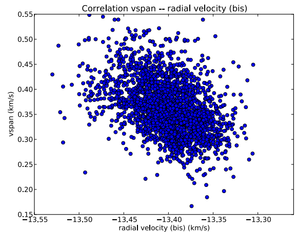
Fig. 9. Anticorrelation of vspan versus vrad (bisector).
