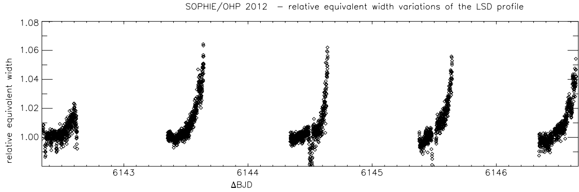
Fig. 12. Nightly relative EW variations of the LSD profiles of this run. Time is expressed in \text{BJD} = 2\,450\,000 + \Delta\text{BJD} .
