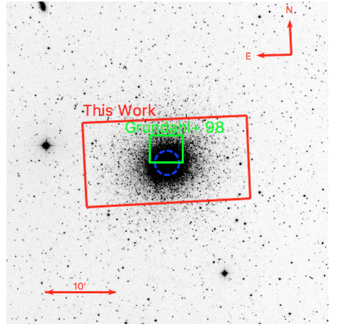
Figure 1. Archival image of M13 from Sloan Digital Sky Survey. The solid red box is the field of view of our data set for WFC chip four. The solid green box is the field of view of NOT observations from Grundahl et al. (1998). The dashed blue circle marks M13 half-light radius.
