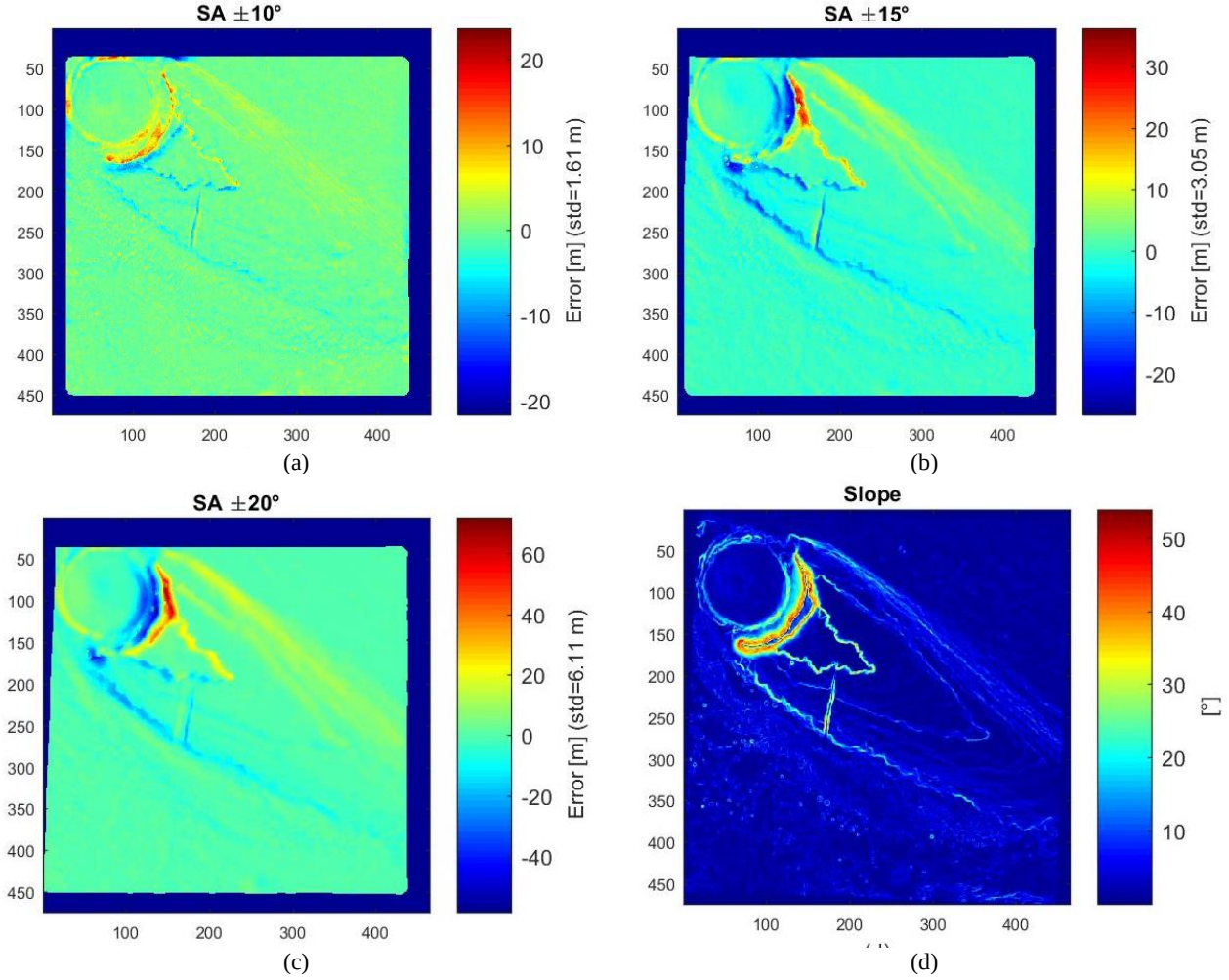
Figure 9 Figures (a), (b), (c) show the Error maps of DTMs generated by the synthetical images respectively with a Stereo Angle (SA) of \pm 10^\circ , \pm 15^\circ , \pm 20^\circ . In (d) the local slope of the reference DTMs is shown.
