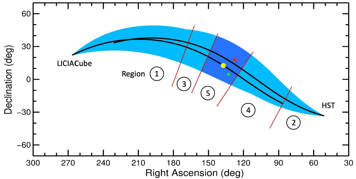
Extended Data Fig. 2 | Ejecta cone orientation lies in the swaths of sky (black lines) defined by HST and LICIACube observations. The light-blue envelope outlines the axis position uncertainty in the direction measured in the sky plane. Red lines divide the along-plane swaths into regions that are excluded based on cone morphology in LICIACube images: 1) and 2) are excluded because the ejecta cone would point in the opposite direction from what is observed; 3) is excluded because the axis would lie too close to the sky plane; 4)
