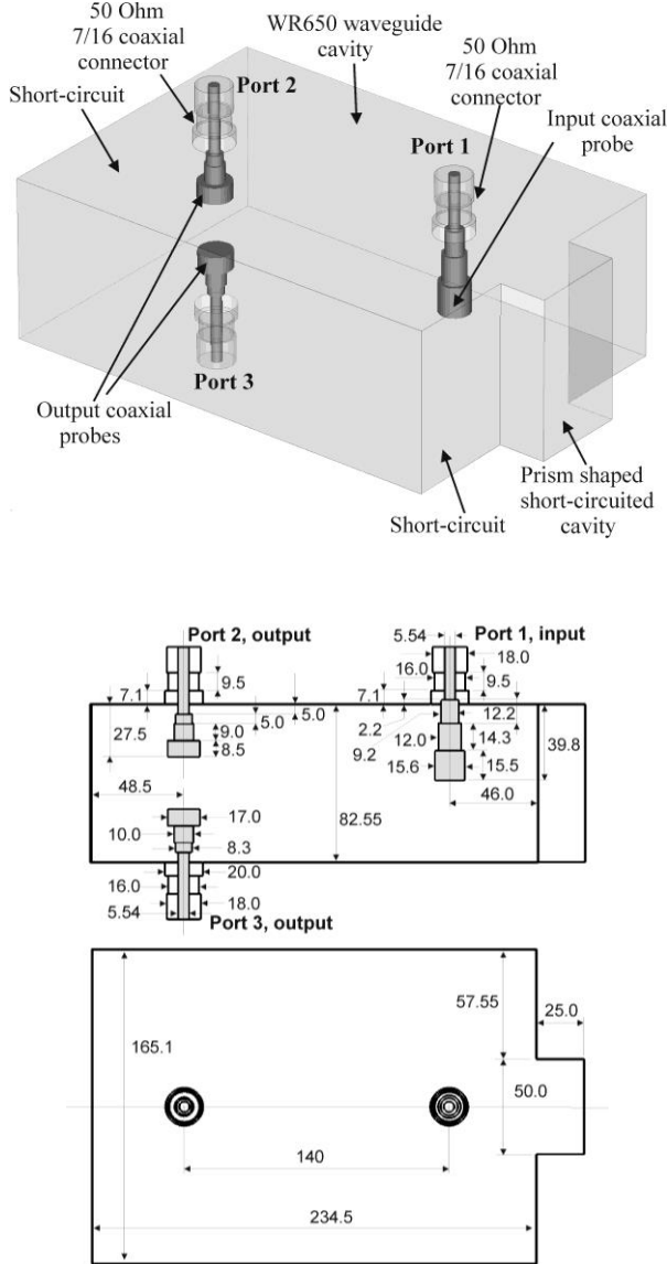
Fig. 1. Top ): Internal 3D view of the waveguide cavity 180^\circ hybrid coupler with 50 \Omega 7/16 coaxial connectors. The length of the hybrid ( \sim 260 \text{ mm} ) is approximately \approx \lambda_g in WR650 waveguide. Bottom ): Cut-out views of the hybrid. Units are in mm.
