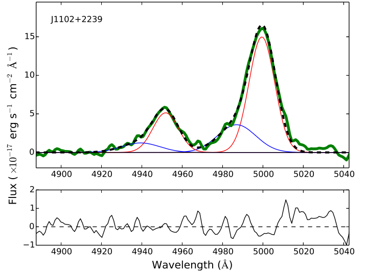
Fig. 3. [O III] lines fitting with the automatic procedure in J1102+2239. Top panel: the thick green line is the original spectrum, continuum and Fe II subtracted. The blue and red solid lines represent the blue wing and core component, respectively. The black dashed line is the sum of the resulting fit. Bottom panel: residuals of the fitting procedure.
