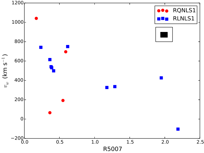
Fig. 13. Distribution of R5007 against the wing velocity in outliers sources with a visible wing. RQNLS1s are indicated by red circles, RLNLS1s are indicated by blue squares. Black filled rectangles as in Fig. 5.
