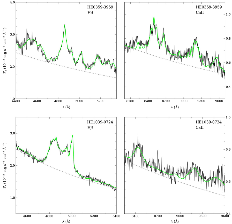
Figure 1. Calibrated spectra with the continuum contribution for H \beta ( left panel ) and Ca II ( right panel ) regions for HE0359-3959 and HE1039-0724. The continuous green line marks the best fit and dashed grey line indicates the continuum level. Abscissae are rest-frame wavelength in Å and ordinates are rest-frame specific flux in units of 10^{-15} \text{ erg s}^{-1} \text{ cm}^{-2} \text{ Å}^{-1} .
