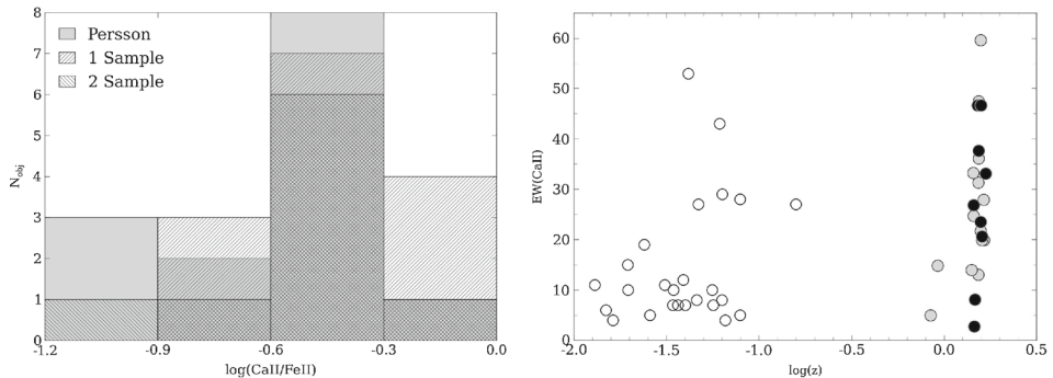
Figure 4. Left panel: Distribution of Ca II/Fe II \lambda 4570 with the newest measurements (1 Sample), Martínez-Aldama et al. 's (2015) sample (2 Sample), and Persson (1988) objects (grey shaded). Right panel: Behavior of the equivalent width of Ca II with respect to redshift. The open circles indicate the Persson's sample, filled circles correspond to Martínez-Aldama et al. 's (2015) sample, and black circles indicate the sample analyzed in this work.
