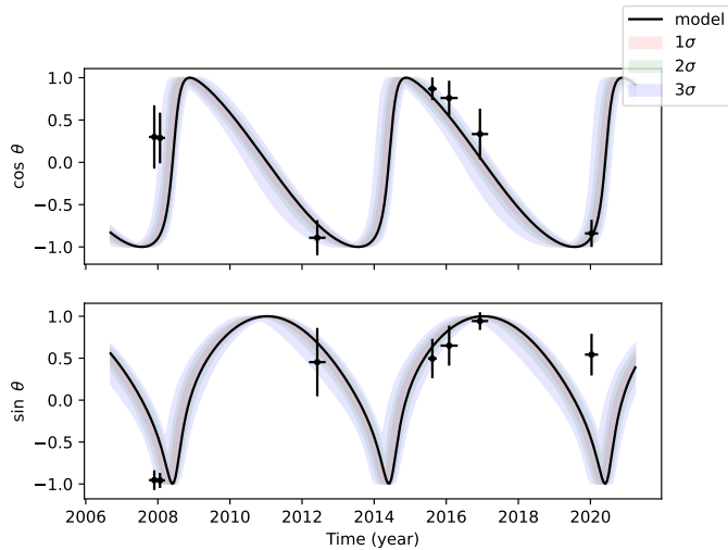
Fig. 7. Simultaneous fit to the sine and cosine of the average position angle, \theta , of the identified VLBI jet features as a function of their computed time of ejection. Most of the points lie within the 3\sigma model uncertainty region. The simultaneous fit avoids the \pm 180^\circ uncertainty in the position angle. The corresponding plot for the position angle, \theta , can be found in Fig. 8.
