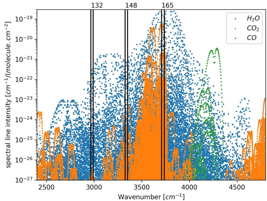
Figure 1. Spectral line intensities in the Nadir and Occultation for Mars Discovery-Solar Occultation spectral range for CO 2 in orange, H 2 O in blue and CO in green. The extension of the main diffraction orders are represented with black vertical lines.
