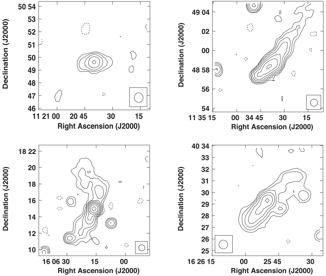
Figure A2. NVSS images of the four sources erroneously included in the FR0CAT catalogue but clearly showing extended radio emission and now excluded from the catalogue: from top left to bottom right panel, SDSS J1120+50, SDSS J1134+48 aka IC 711, SDSS J1606+18 and SDSS J1625+40. The contour levels of the maps are (-1, 1, 2, 4, 8, \dots) mJy beam -1 .
