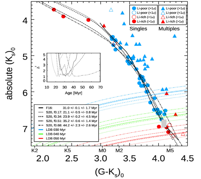
Figure 5. Similar to Fig. 4 but showing the loci of constant luminosity for 99 per cent Li depletion (coloured lines), the best-fitting isochrones (black lines) and \chi^2_r versus age for a series of magnetic models (see Section 4.2).
