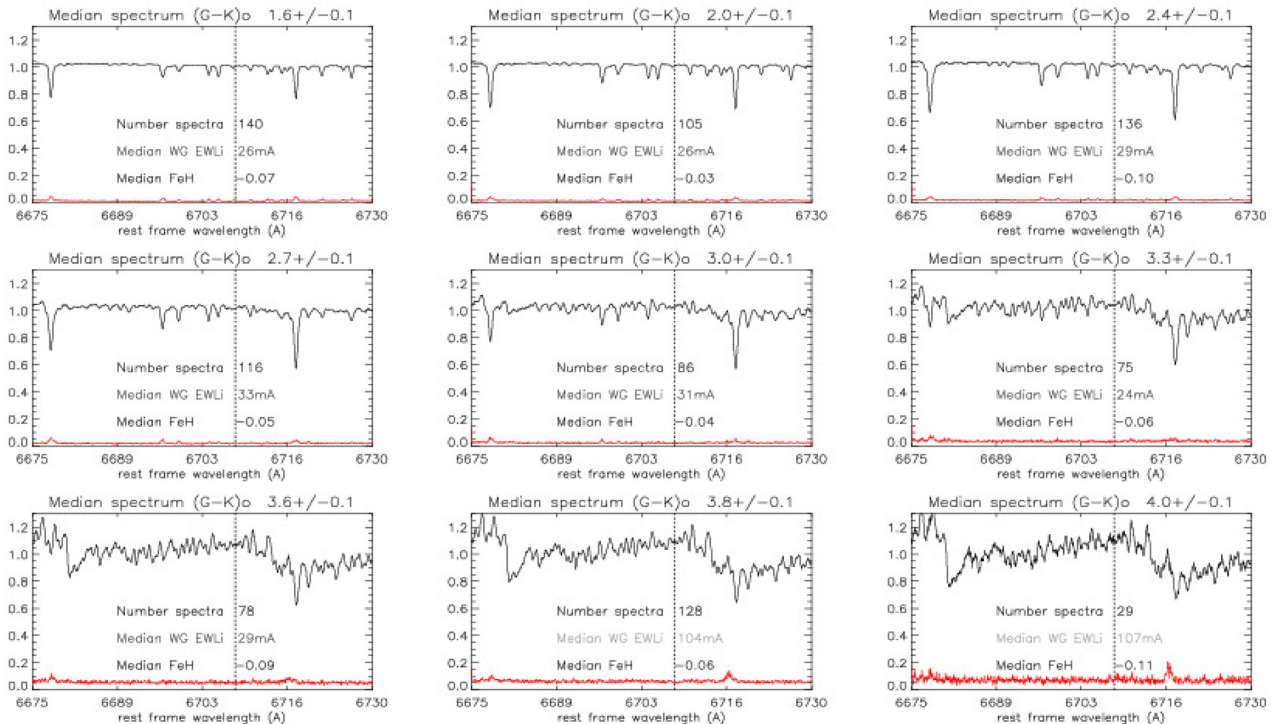
Figure B2. Examples of median continuum spectra for stars with low levels of Li as a function of (G - K_s)_0 . Text on each plot shows the number of spectra averaged in each bin and median values of EW(Li) and [Fe/H]. The lower red curve shows the uncertainty in the continuum waveform, calculated as 1.3 times the median absolute deviation of individual spectra from the median spectrum. The dotted line indicates the position of the Li I 6708 Å absorption line.
