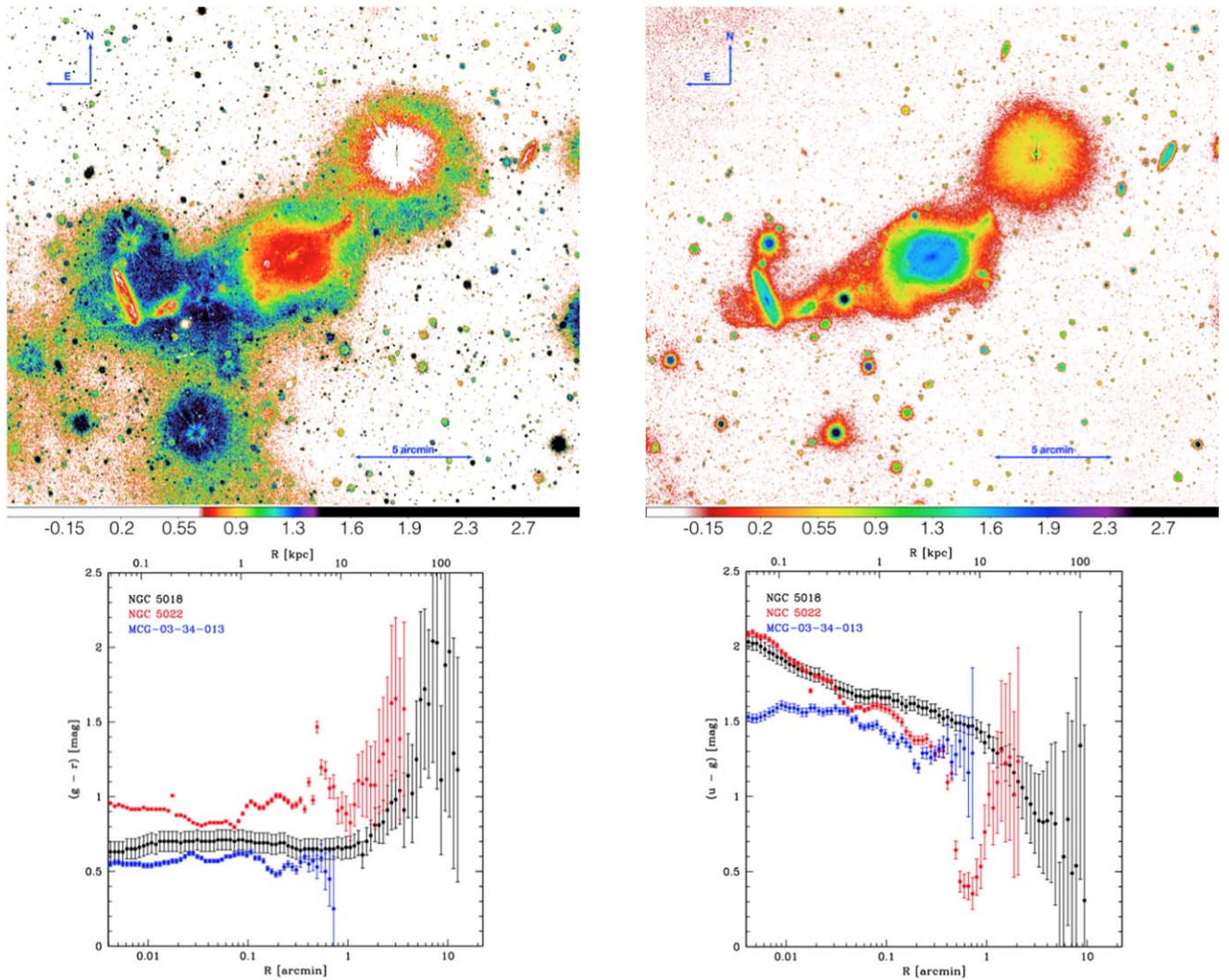
Figure 7. (g-r) (top-left panel) and (u-g) (top-right panel) color maps centered on NGC 5018. Bottom: azimuthally averaged, extinction-corrected, (g-r) (left) and (u-g) (right) color profiles of NGC 5018 (black), NGC 5022 (red), and MCG-03-34-013 (blue).
