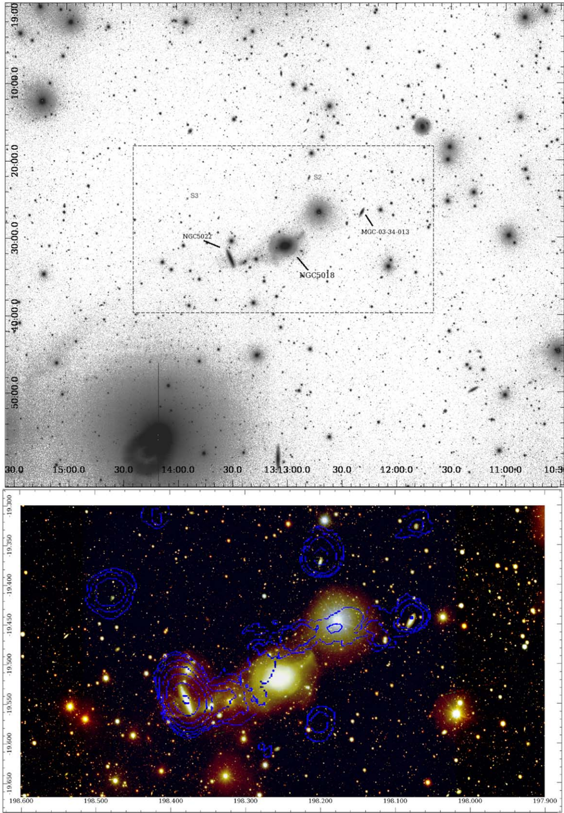
Figure 1. Top: VST g -band mosaic of the NGC 5018 group. The image size is 1^{\circ}2 \times 1^{\circ}0 . Bottom: color composite image of the central regions of the group ( 0^{\circ}7 \times 0^{\circ}4 ), assembled from u -, g -, and r -band VST images, with the H I map from the Very Large Array (VLA) superimposed (blue contours), adapted from Kim et al. (1988).
