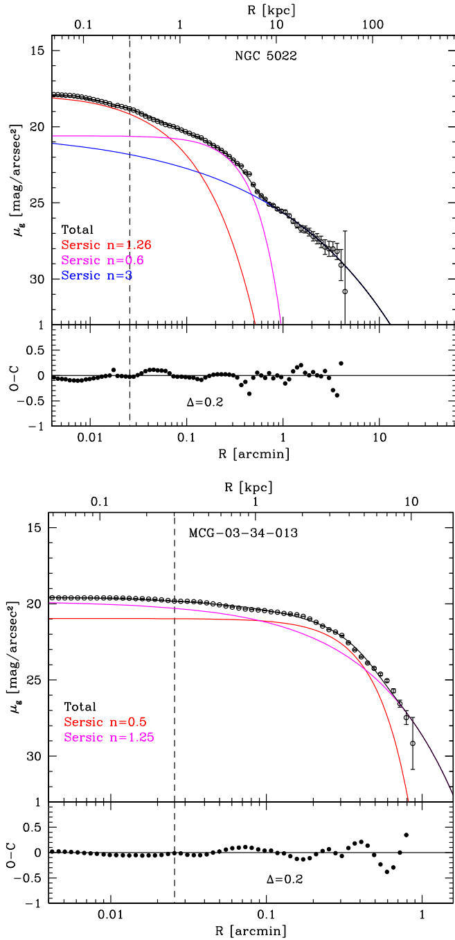
Figure 14. VST g -band profiles of NGC 5022 (top), fitted with a three-component model, and MCG-03-34-013 (bottom), fitted with a double Sérsic model.
