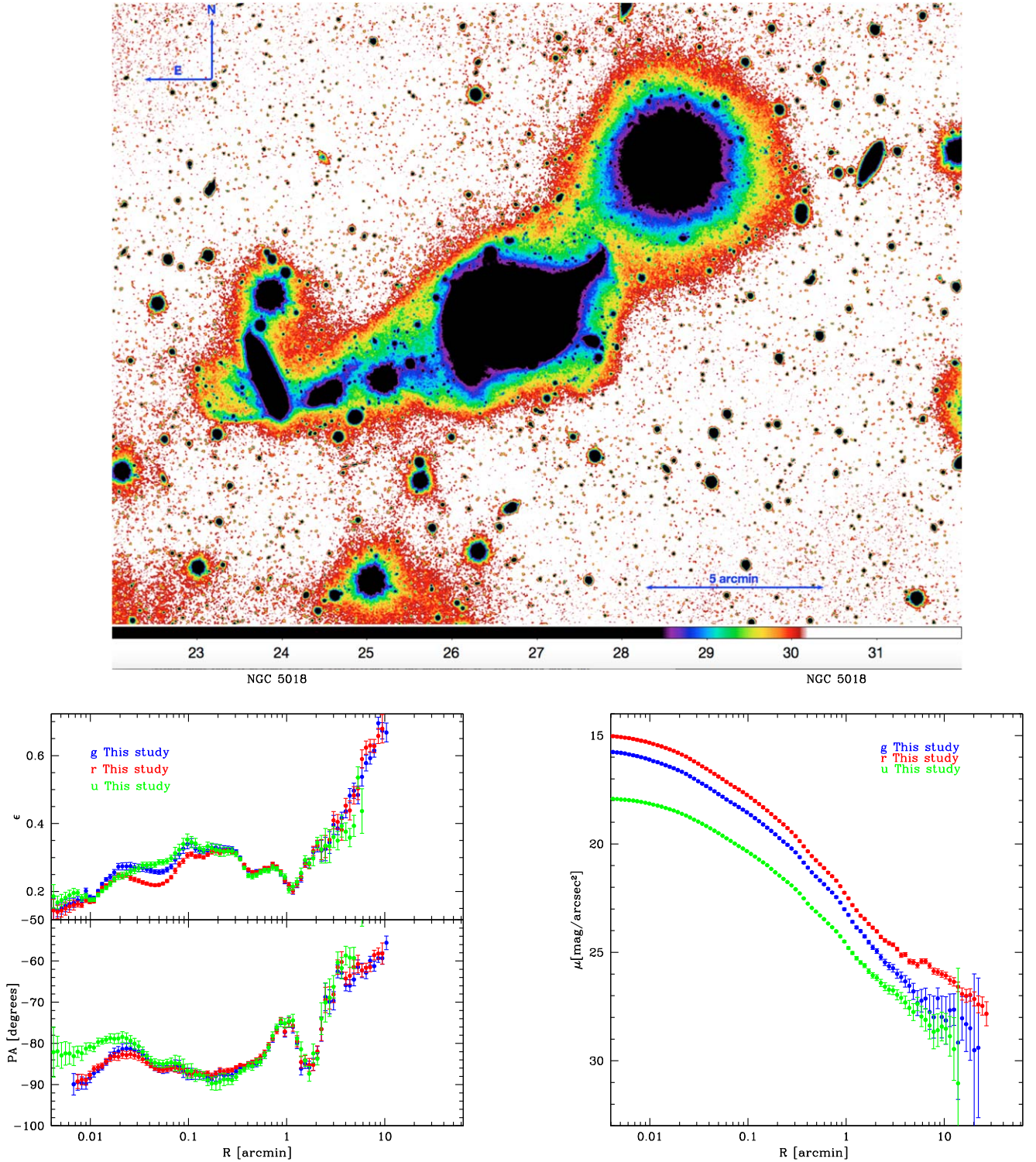
Figure 2. Top: VST g -band sky-subtracted image of the 0.4 \times 0.4 field around NGC 5018. The color scale represents surface brightness in \text{mag arcsec}^{-2} . Bottom left: ellipticity ( \epsilon ) and position angle (P.A.) profiles for NGC 5018, in the g band (blue points), r band (red points), and u band (green points). Bottom right: azimuthally averaged surface brightness profiles in the g (blue), r (red), and u (green) bands.
