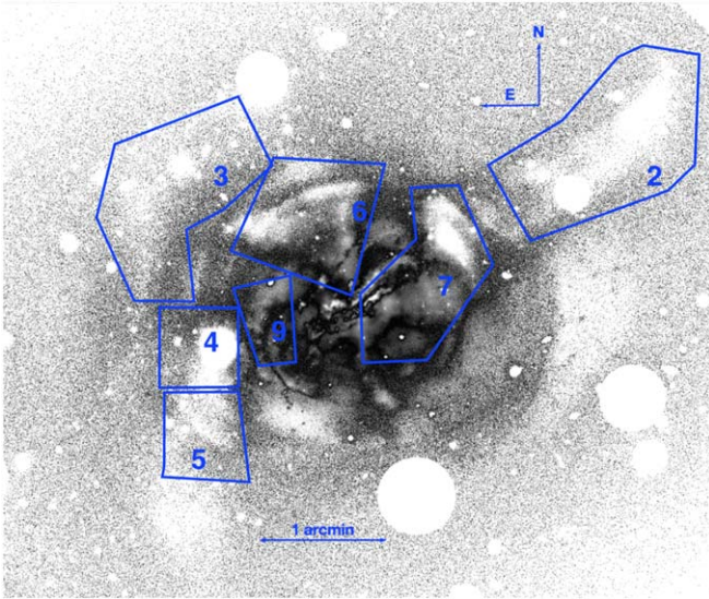
Figure 6. Result of the model-fitting and division method employed to quantify the tidal disturbance of NGC 5018 (see text). The image size is 6 \times 5 \text{ arcmin}^2 . The overplotted blue contours mark the substructures shown in Figure 5, which are also visible in this image.
