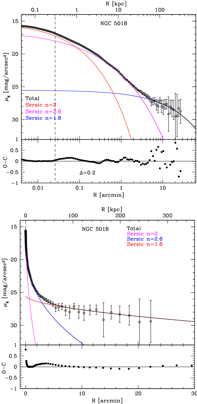
Figure 13. VST g-band profile of NGC 5018, on a logarithmic scale (top) and a linear one (bottom), fitted with a three-component model motivated by the predictions of theoretical simulations (see Spavone et al. 2017). The dashed line indicates the core of the galaxy, which was excluded in the fit.
