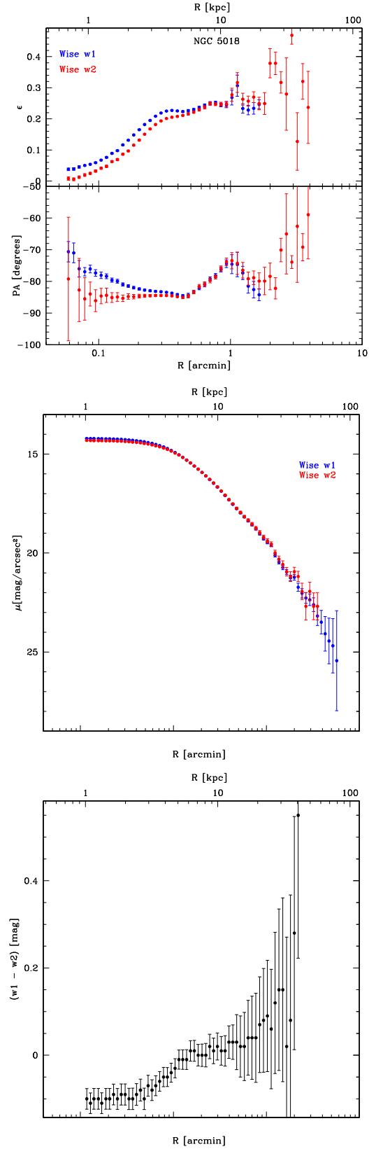
Figure 9. Top: ellipticity ( \epsilon ) and position angle (P.A.) profiles for NGC 5018, in the WISE w1 ( 3.368 \mu\text{m} , blue points) and w2 ( 4.618 \mu\text{m} , red points) bands. Middle: azimuthally averaged surface brightness profiles in the w1 and w2 bands. Bottom: azimuthally averaged color profile.
