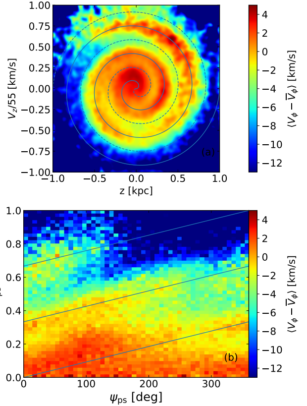
Figure 6. Kinematic properties of stars in the solar neighbourhood using data from Gaia DR2. Stars were selected to be within |R - R_0| < 1.0 kpc and |\phi - \phi_0| < 15^\circ . Top: map of \langle V_\phi(z, V_z) \rangle - \bar{V}_\phi with the volume-weighted median value ( \bar{V}_\phi = 228.3 km s -1 ) subtracted. The archimedean spirals are defined in equation (3). Bottom: the unwound spiral pattern as a function of r_{ps} (dimensionless) and \psi_{ps} (in degrees). The three diagonal lines wrap around every 2\pi and thus correspond to three different r_{ps} intervals in the zV_z plane. Note the underlying velocity gradient in r_{ps} due to the asymmetric drift.
