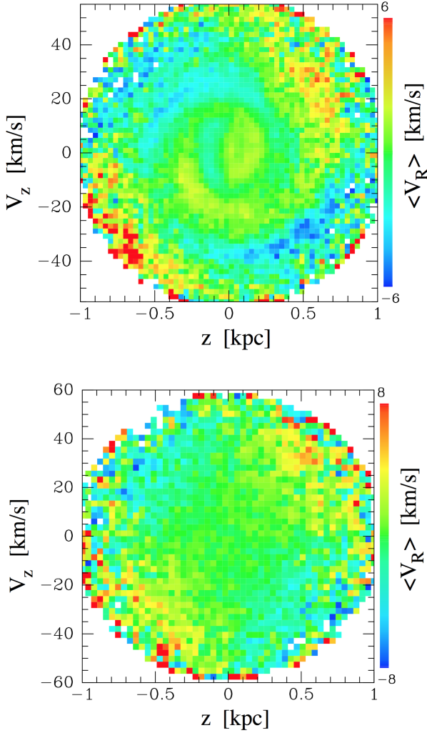
Figure 15. Top: \langle V_R \rangle plotted in the zV_z phase plane over the original volume explored by Antoja et al. (2018). A quadrupole pattern (blue top left and bottom right, red bottom left and top right) dominates the outer portion of the circle. Towards the centre, the spiral is clearly visible. Bottom: The simulated zV_z plane in a realistic axisymmetric model Galaxy (with no perturbing force) using 10^6 particles with sampling to match the Gaia selection function. The same quadrupole is apparent and arises because of the tilt of the velocity ellipsoid.
