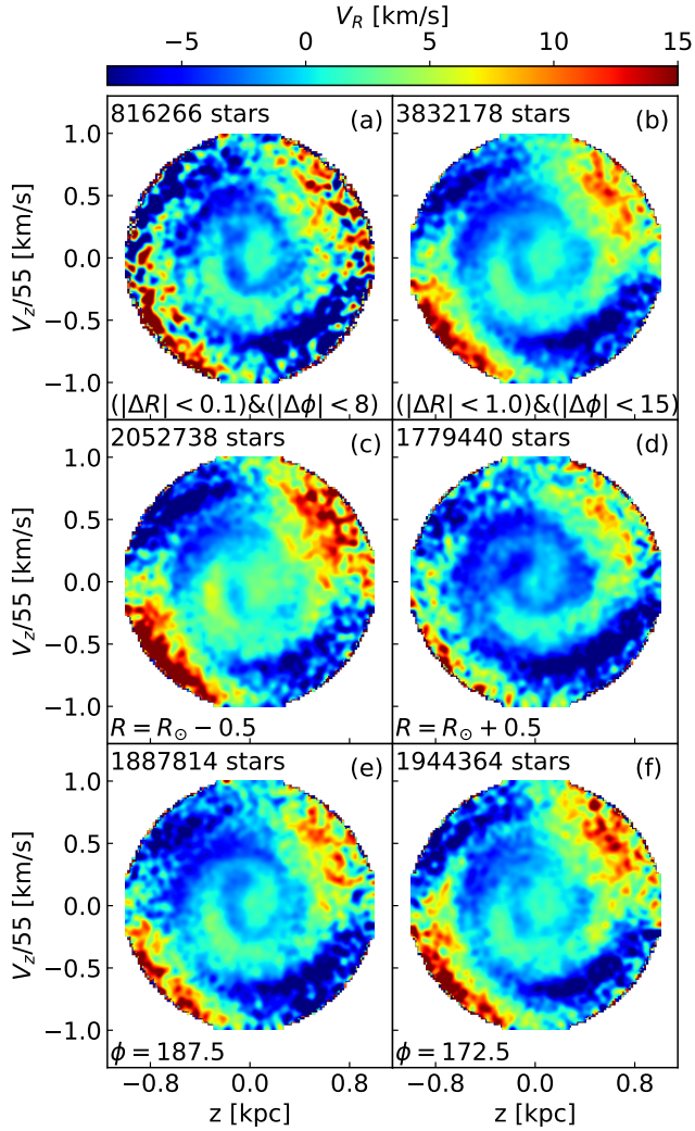
Figure 17. Map of median V_R in (z, V_z) plane for stars in the solar neighborhood using data from Gaia DR2. The sample definitions are the same as in Figure 8. The quadrupole defined by the sign changes in each quadrant are due to the tilt of the velocity ellipsoid (see the sketch in Figure 16). Note that a weak phase spiral is visible in the center. The pattern is stronger for the R = R_0 - 0.5 case than for the R = R_0 + 0.5 case. ( \phi is quoted in degrees.)
