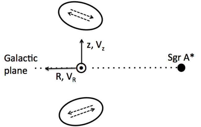
Figure 16. (Left) The adopted coordinate frame in Galactic cylindrical coordinates shown with respect to the Sun's position. The tilted velocity ellipsoids above and below the Galactic plane are also indicated. The dashed arrows show the direction of the fastest motions within the ellipsoid. When viewed from the Sun, the velocity ellipsoids produce a characteristic quadrupole \mp pattern seen in the \langle V_R(z, V_z) \rangle plane from the GALAH and Gaia data.
