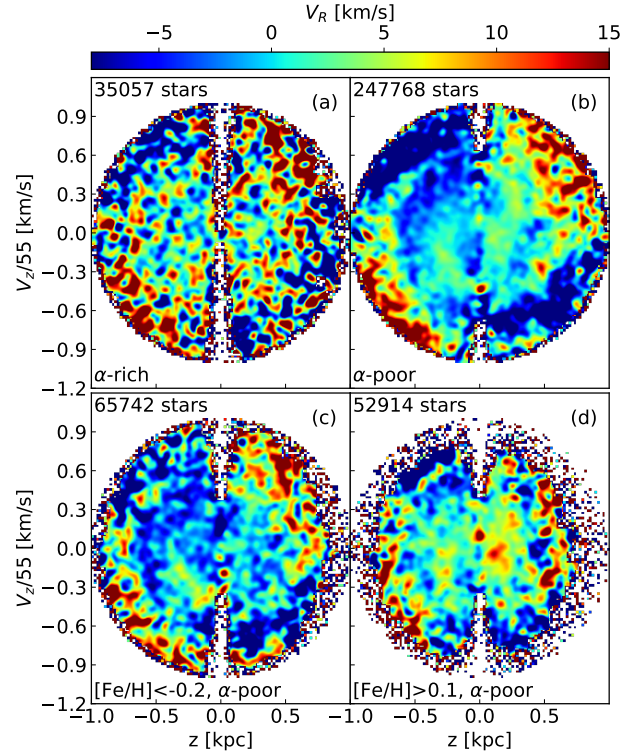
Figure 18. Map of median V_R in (z, V_z) plane for stars in the solar neighborhood using data from GALAH and Gaia DR2. The sample definitions are the same as in Figure 10.
