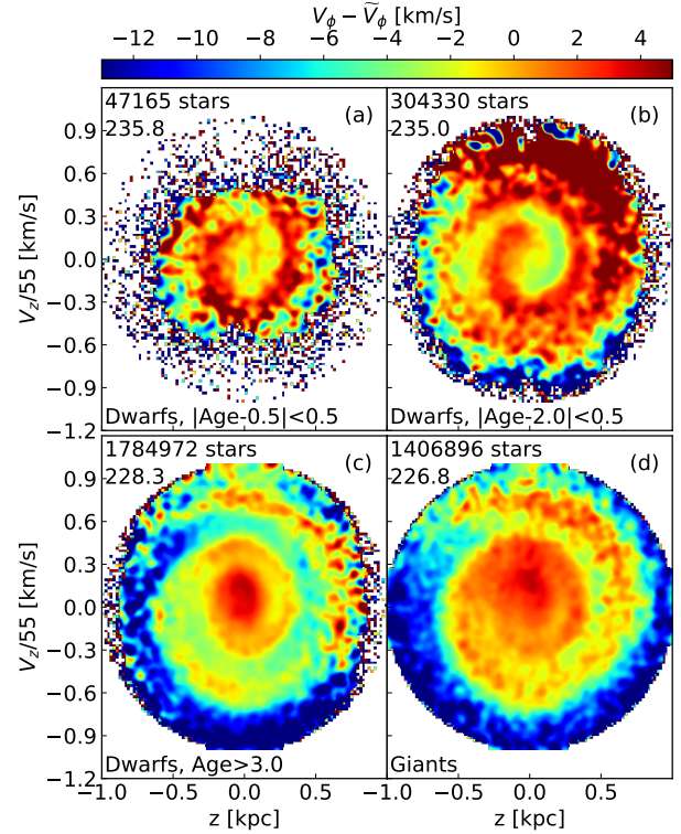
Figure 14. An analysis of the Gaia photometry over the GALAH volume in the zV_z plane showing crude stellar ages for (a–c) dwarfs and (d) giants. Stars younger than about 3 Gyr emphasise the ‘hook’ at the centre of the phase spiral (a,b). This feature closely resembles Figure 11b for which J_R < 0.01 , i.e. younger stars from the local disc are on more circular orbits. The old dwarfs (c) and giants (d) resemble Figure 11a for which J_R > 0.01 , i.e. the older stars are on more elliptical orbits.
