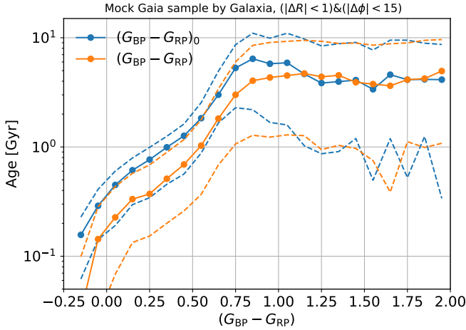
Figure 13. Given the assumed model and selection function for the Galaxy of Figure 12, we derive a mean stellar age as a function of the Gaia colour for the dwarf stars. The lower solid curve is based on the raw Gaia photometric data uncorrected for dust extinction; the 16 and 84 percentile ranges are shown as dashed lines. The upper curves are the Gaia photometric data corrected for dust extinction. Age discrimination is impossible beyond about 3.5 Gyr.
