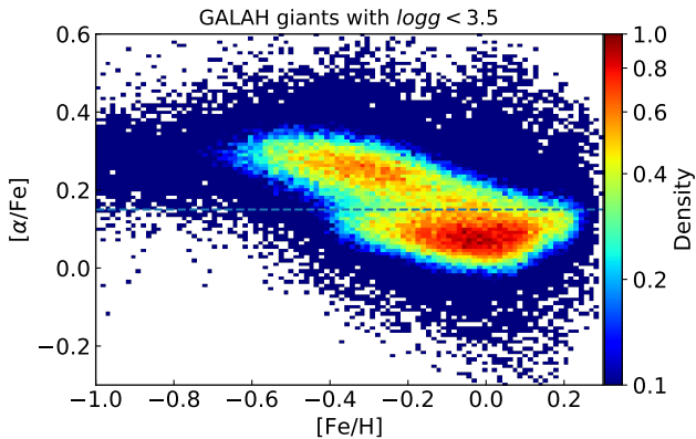
Figure 3. Normalised density of giants in the [\text{Fe}/\text{H}] vs. [\alpha/\text{Fe}] plane using data from the GALAH survey ( \log g < 3.5 ). A clear separation of the high and low [\alpha/\text{Fe}] populations is visible. The dashed boundary line distinguishes the high and low [\alpha/\text{Fe}] populations (cf. Adibekyan et al. 2012). The simple choice of boundary is vindicated in Section 4.3 where we show that the dynamical properties (actions) of the high and low [\alpha/\text{Fe}] populations are distinct.
