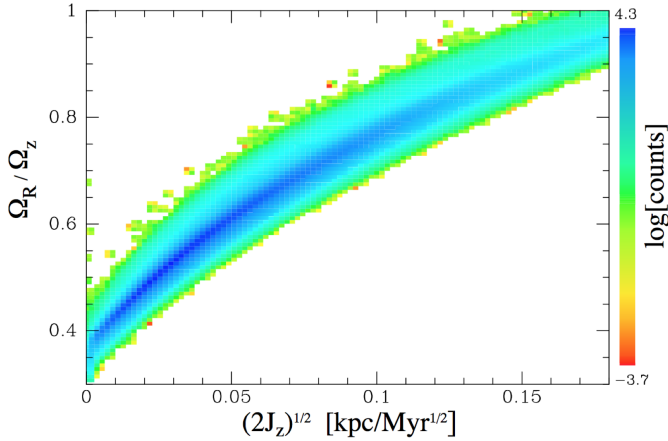
Figure 5. The frequency ratio \Omega_R/\Omega_z vs. \sqrt{2J_z} for orbits calculated in a realistic Galactic potential; the ratio for most stars lies in the range 0.5 – 0.7. The factor 2 in front of J_z ensures that the area inside a curve of constant J_z is 2\pi J_z in the zV_z plane. Note that a range of frequencies operates in R and z for all values of J_z .
