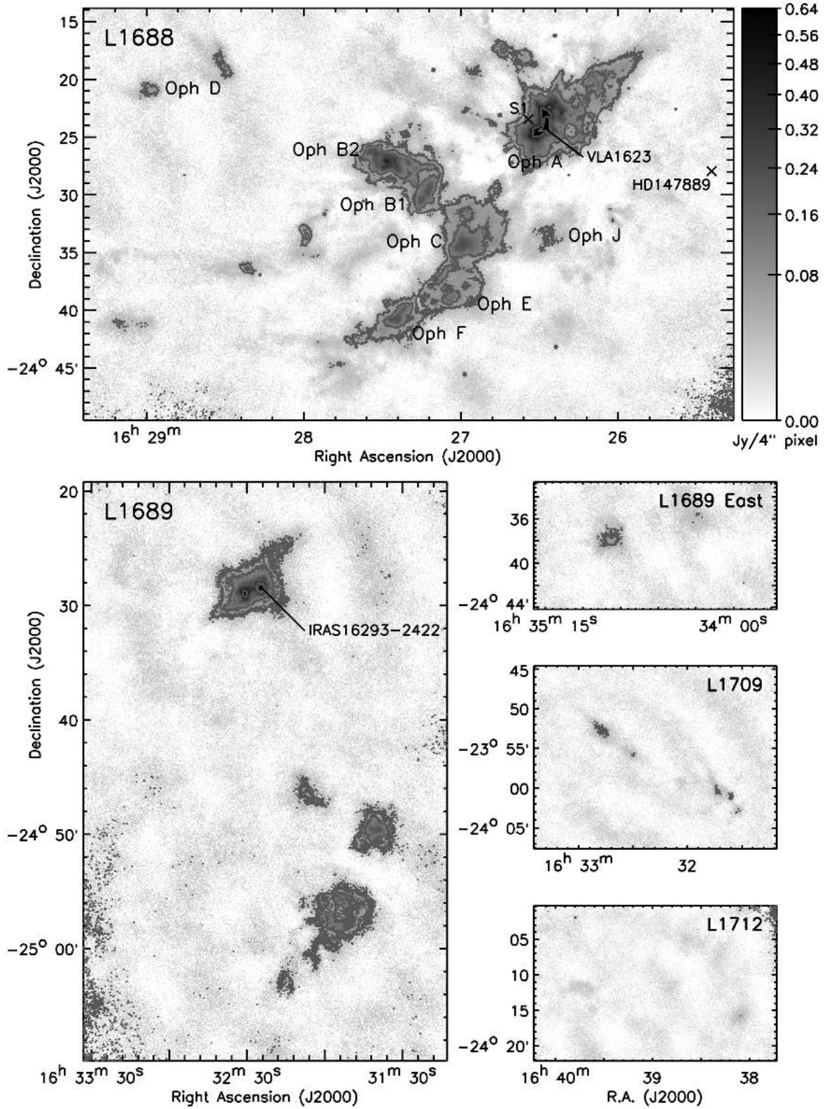
Figure 2. 450-μm flux density data, shown in square-root scaling, for each of the subregions of Ophiuchus (see text for details). The B stars HD 147889 and S1 are marked, along with the Class 0 protostars VLA 1623 and IRAS 16293–2422. The subregions of the L1688 cloud are labelled.
