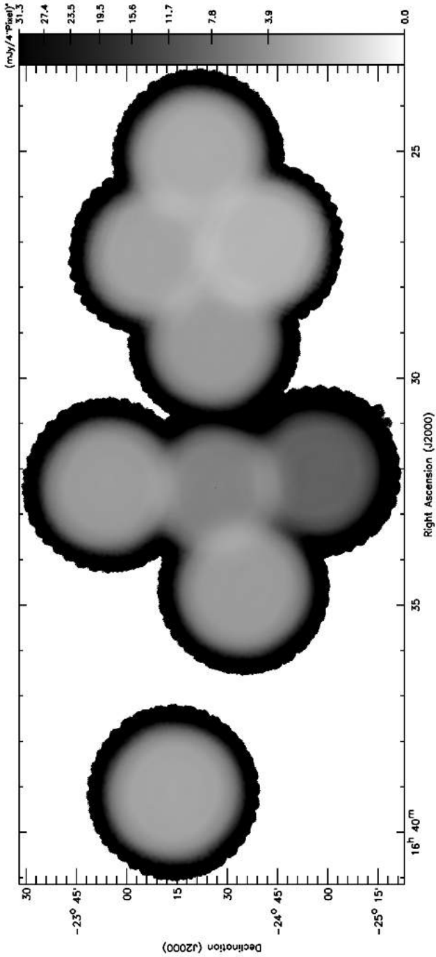
Figure A4. The variance on the SCUBA-2 450- \mu m flux density data, shown in square-root scaling.
