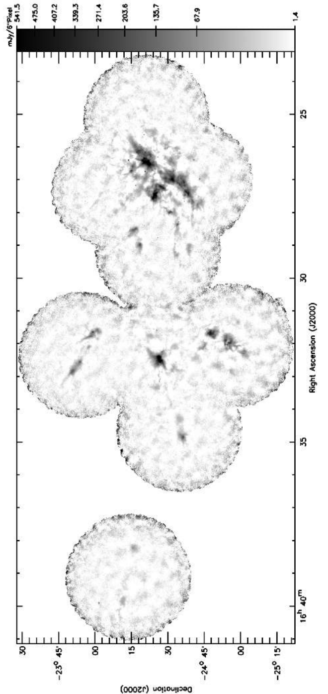
Figure A1. The 850- \mu m flux density measured in Ophiuchus with SCUBA-2, shown in square-root scaling.
