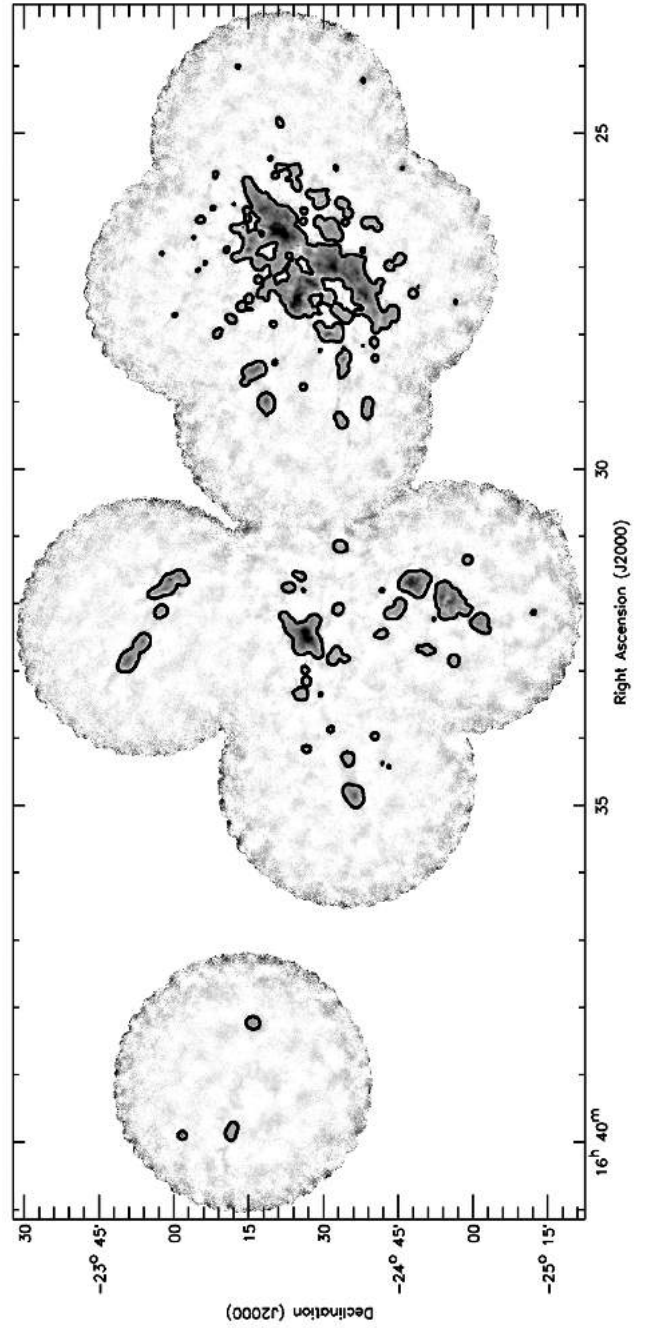
Figure A5. The mask used in the data reduction process, enclosing regions of significant emission, shown as a thick contour, overlaying the 850- \mu m flux density data, shown as a grey-scale.
