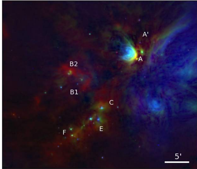
Figure 12. Three-colour image of L1688, with regions labelled. Red channel: SCUBA-2 850 \mu\text{m} data (this work). Green channel: Herschel 100 \mu\text{m} data (Ladjelate et al., in preparation). Blue channel: Spitzer 8 \mu\text{m} data (Evans et al. 2003).
